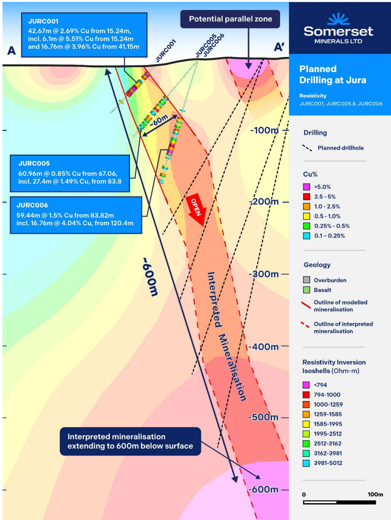
Figure 1: Cross-section at Jura showing planned drilling targeting down-dip to JURC001 (42.7m @ 2.69% Cu from 15.24m), as well as potential parallel mineralised structures. Interpreted mineralisation extends to ~600m below surface and remains open. See ASX:SMM 04/02/2026.
