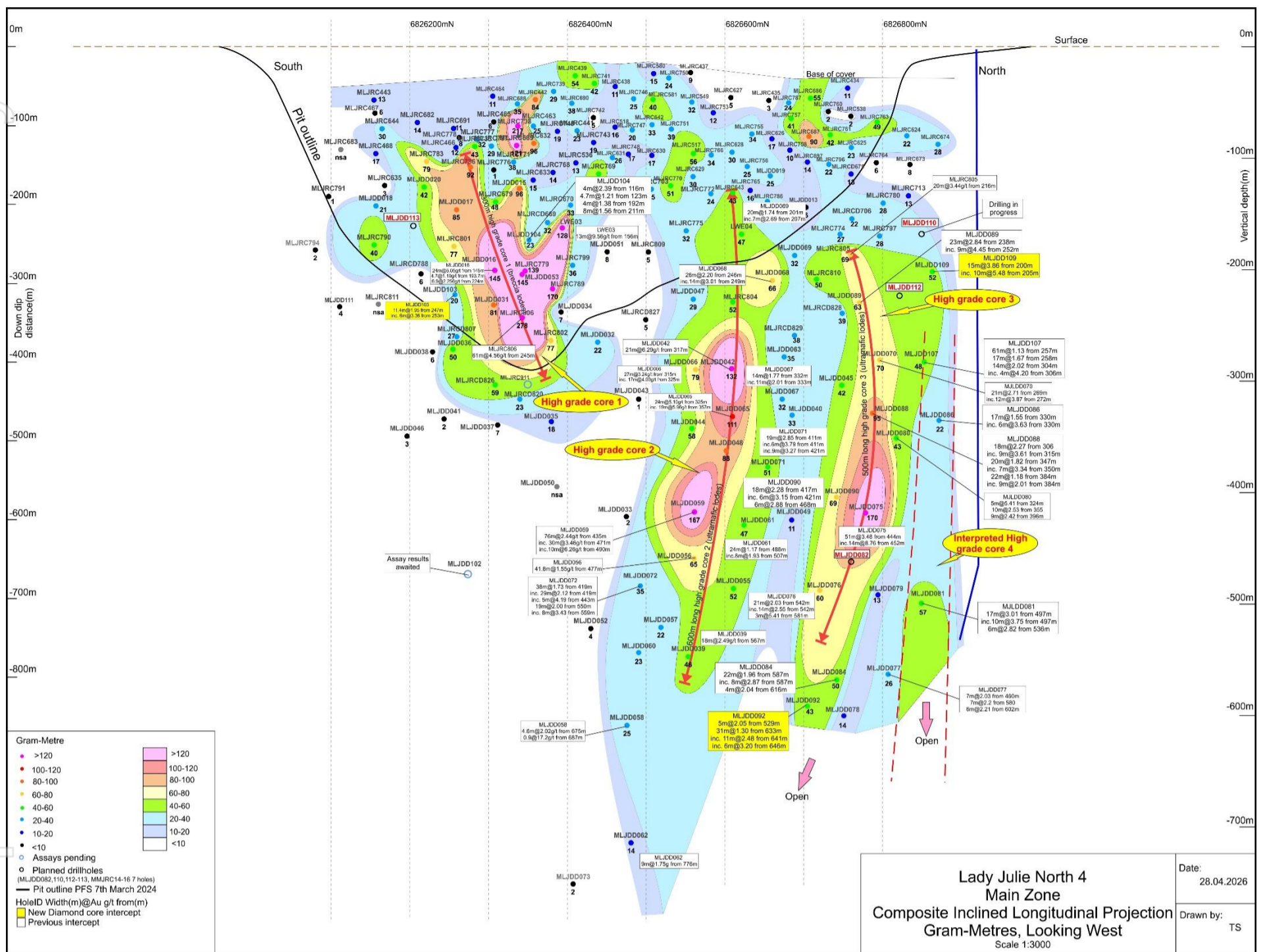
Figure 1. Composite Inclined longitudinal projection of the main lode in LNJ4 in gram-metres. Highlighting continuous mineralisation over the whole 750m strike length. Four high grade core zones have been defined. The southern High-Grade Core Zone 1 is 300 x 200m in size and is associated with multiple silica pyrite and breccia lodes and is being further tested with MLJDD113. High-grade Core zone 2 is 150m x 600m and is associated with altered silicified and fuchsite ultramafic lodes. HGC3 is 150m x 600m and has similar alteration as HGC2. High-Grade Core 4 is 100m x 500m and has similar alteration as HGC3 and remains open at depth, and is currently being tested with further infill holes MLJDD085, MLJDD110 and MLJDD112.
