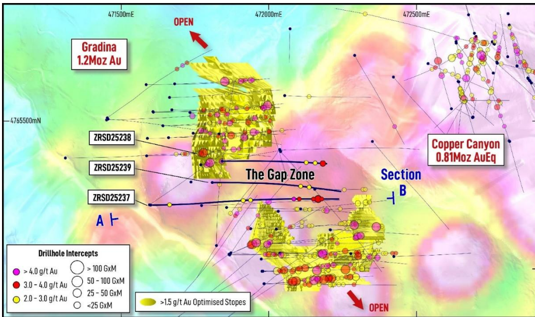
Figure 3. Plan view map of the Gradina and Copper Canyon Deposits, showing drill traces, drill-hole intercepts, gold-arsenic soil geochemical response. 3
