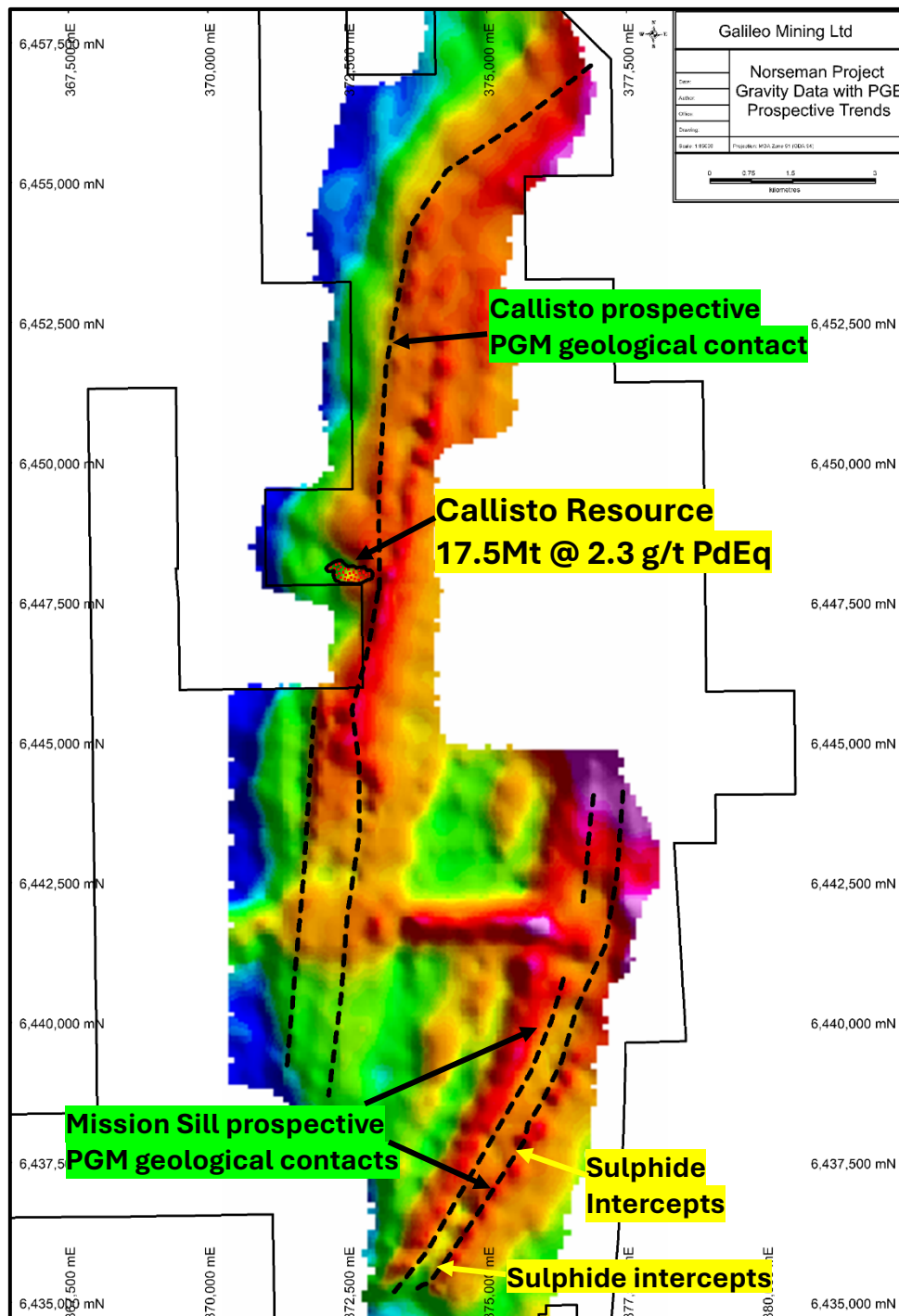
Figure 4 – Norseman Project residual gravity image with PGM prospective geological contacts, existing Callisto resource, and recent sulphide intercepts 1 at the Mission Sill prospect.
