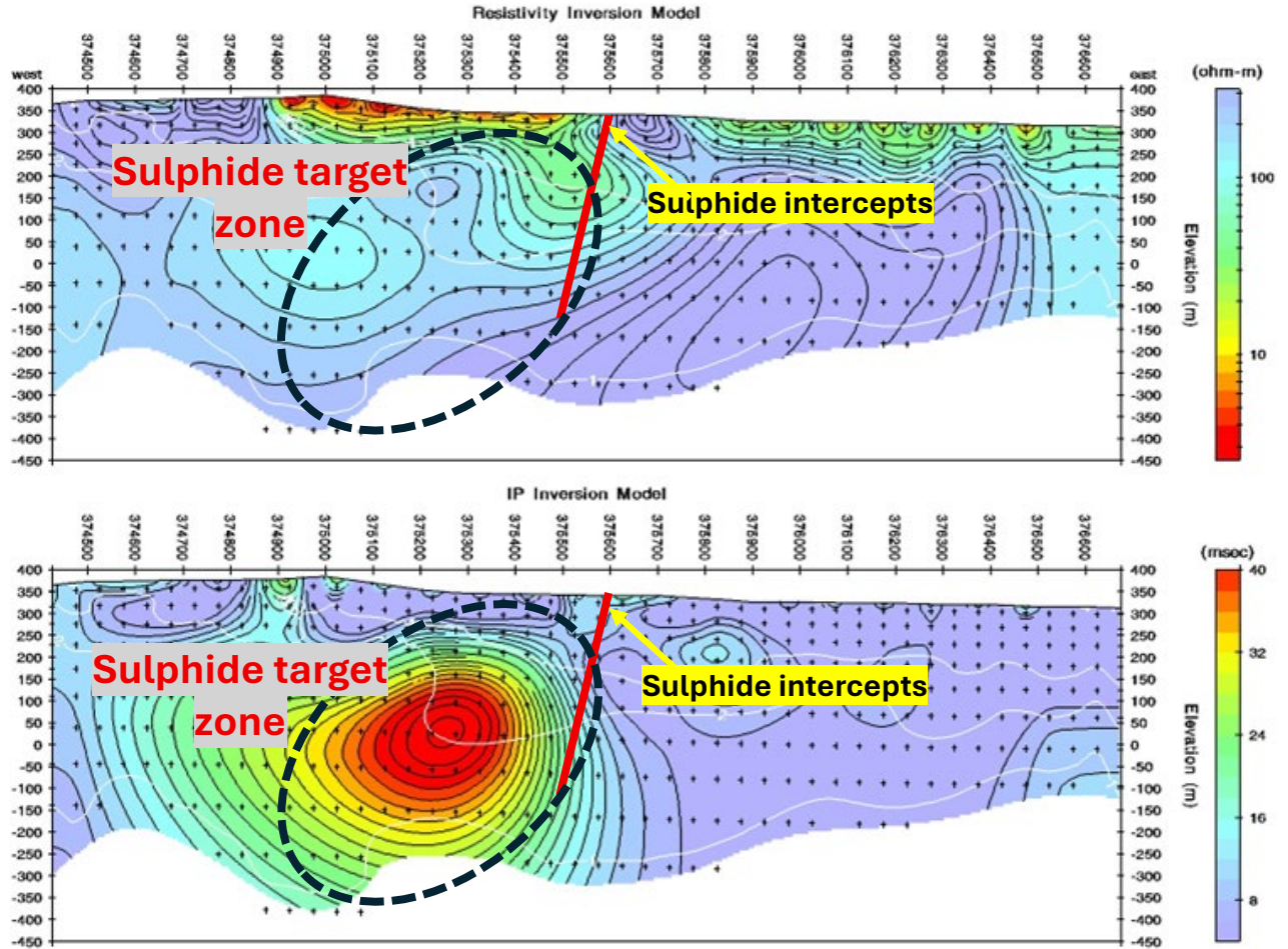
Figure 3 – Mission Sill section 6,437,800N with sulphide target zones at depth.
