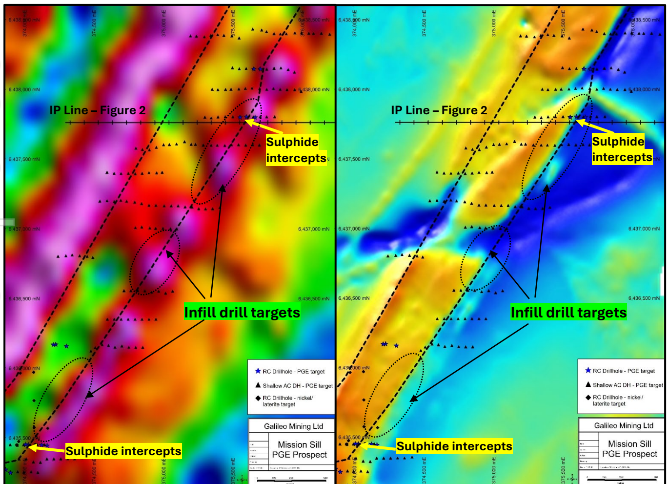
Figure 1 – Mission Sill Prospect sulphide intercepts, PGE target horizons (dashed lines), infill drilling targets (ellipses), with detailed 1VD gravity image (left) and TMI magnetic image (right).
