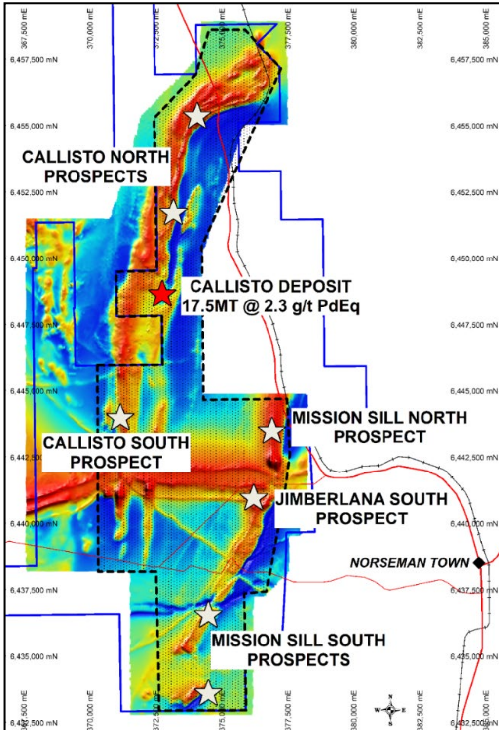
Figure 5 – Norseman Project outline (blue line) with PGE prospective area (black dashed line), Callisto Deposit (red star), and prospects (grey stars).
