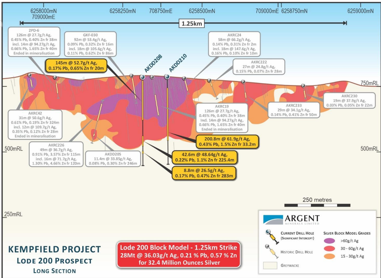
Figure 4 – Long Section over Lode 200 showing current drill holes & historical mineralised intercepts.
