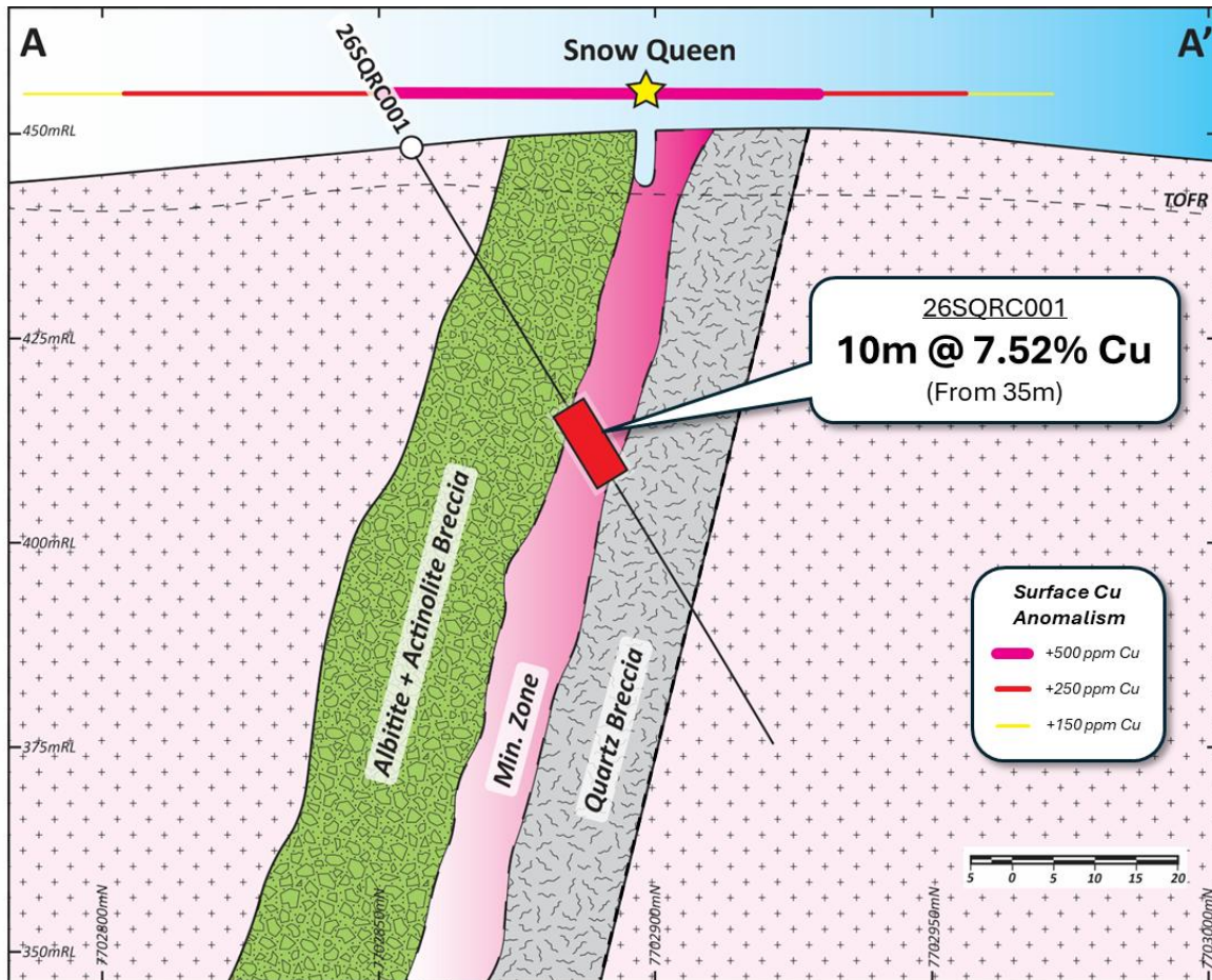
Figure 2: Cross-section through 26SQRC001
