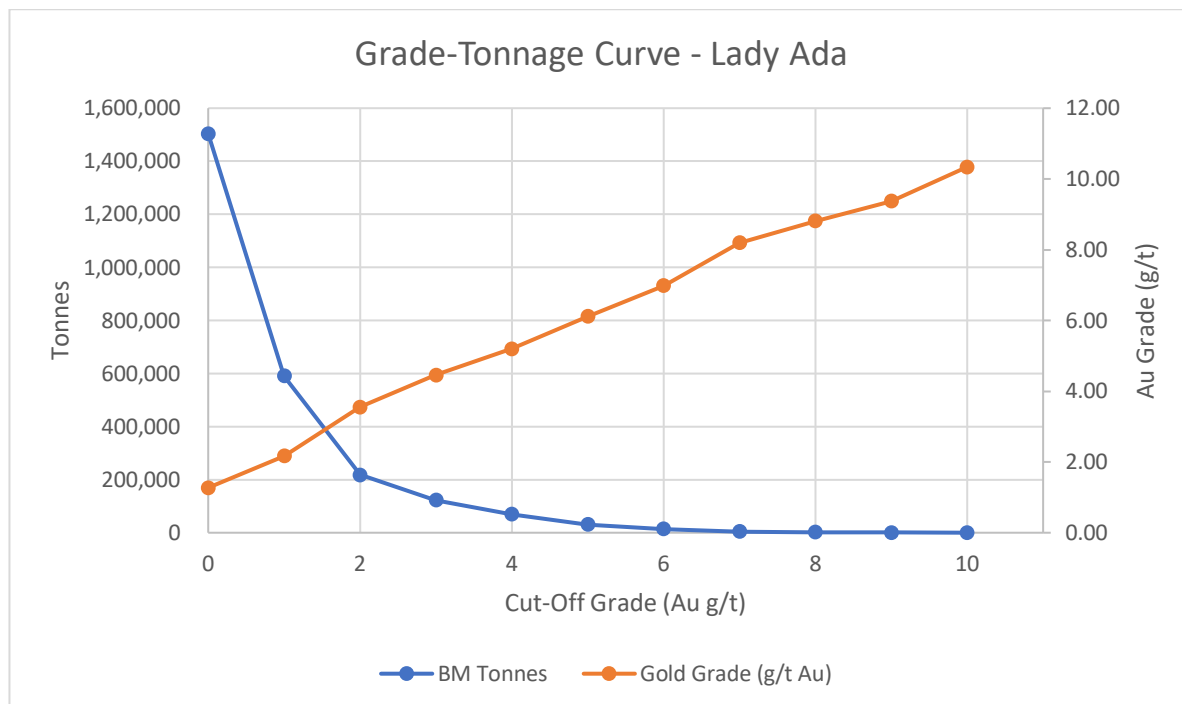
Figure 11 – Lady Ada Grade-Tonnage Curve
