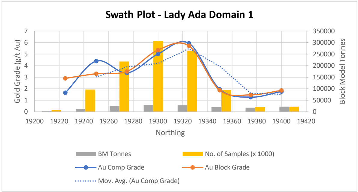
Figure 8 - Swath Plot by Northing – Lady Ada Domain 1
