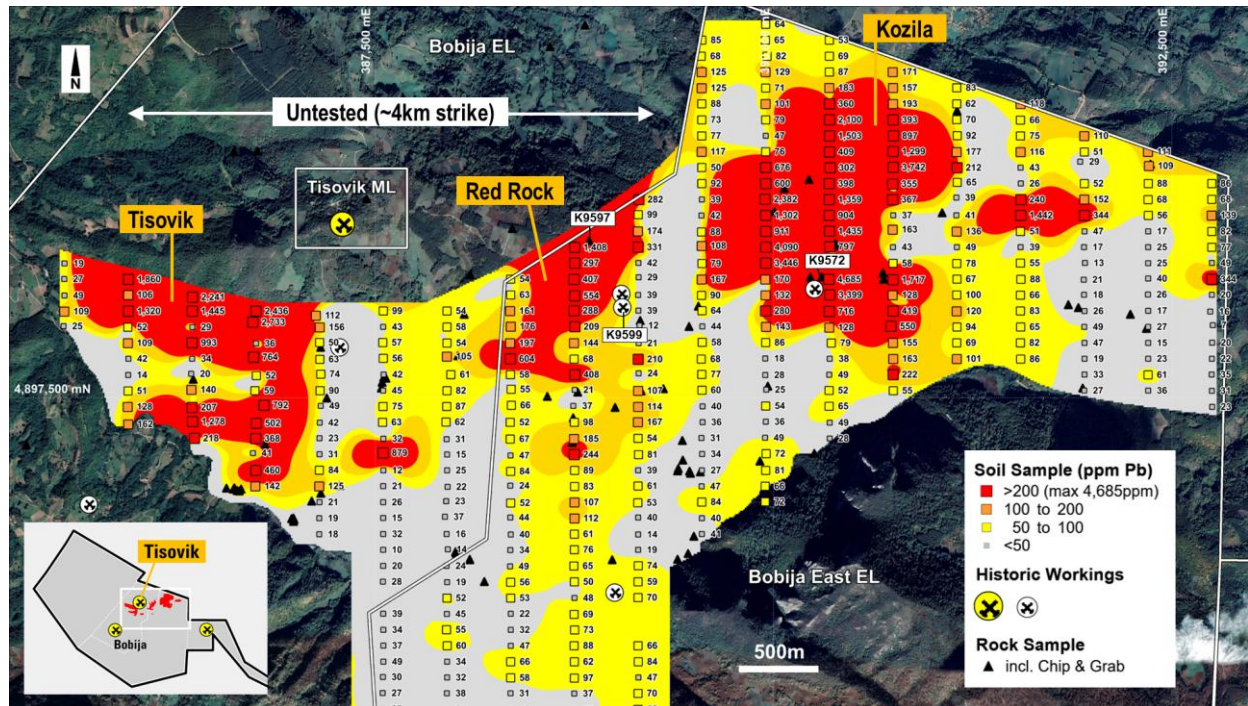
Figure 2: Soil sample lead results in the Tisovik area showing expanded Kozila Anomaly and multiple zones of interpreted +200ppm lead-in-soil anomalism, with rock samples locations, and location of historic workings.
