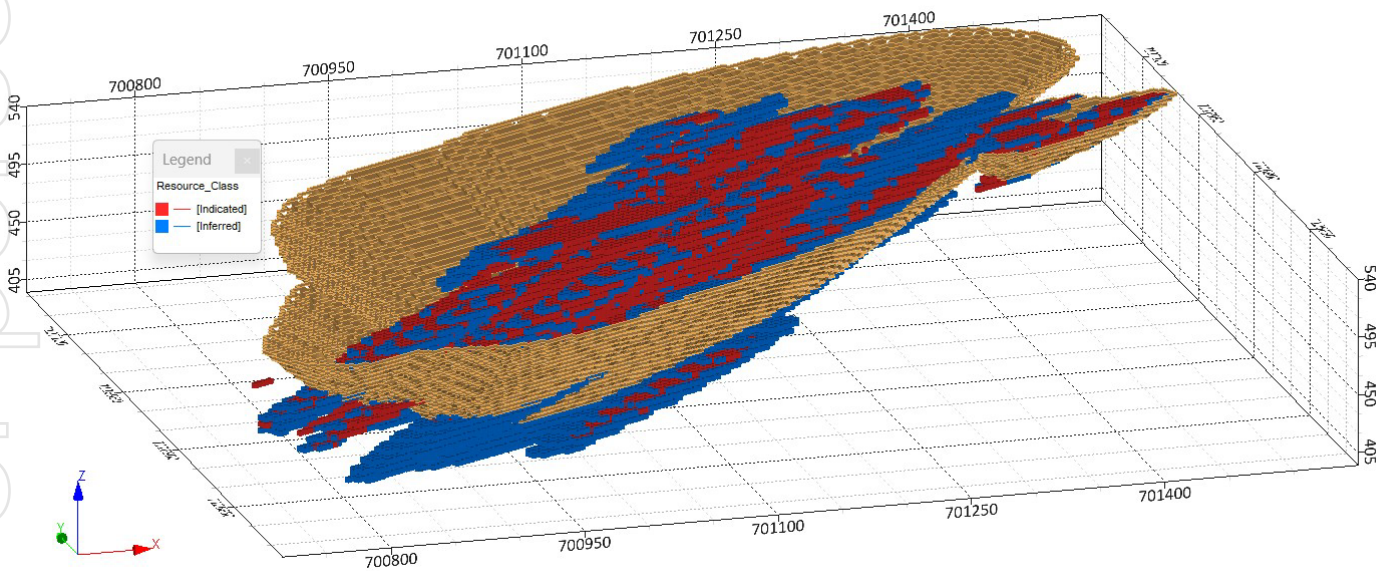
Figure 13: Plan view of the Big John Au grade-constrained block model and optimised pit shell (top). 3D block model of the Big John deposit illustrating resource classification within the optimised open pit shell (bottom), the green Y-axis denotes north
