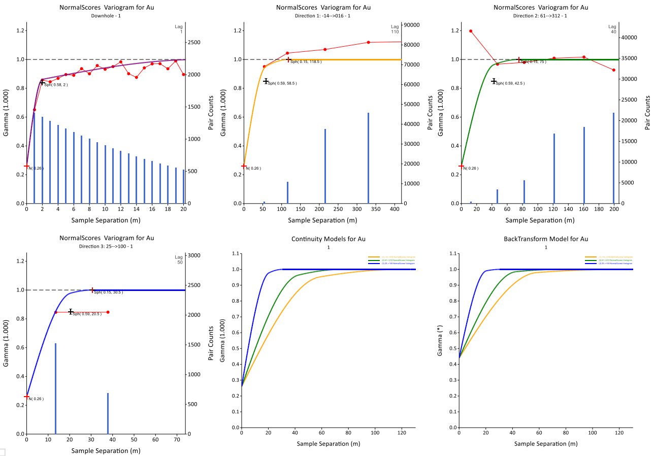
Figure 6: Experimental Variograms and fitted models BDT2 Object 1
