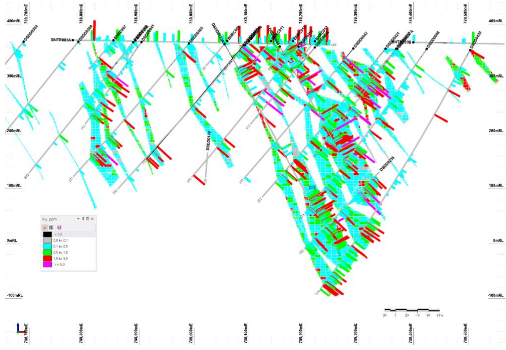
Figure 8: Example cross section (1,059,625mN) BDT2 showing estimated gold grades and drill data (looking north +/-25m)
