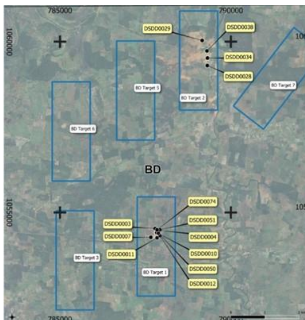
Figure 10: Location of the Diamond Drill Collars used for the Metallurgical Composites
