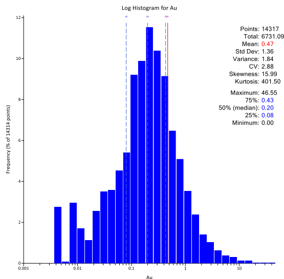
Figure 5: Log histogram for BDT2 composites (all)
