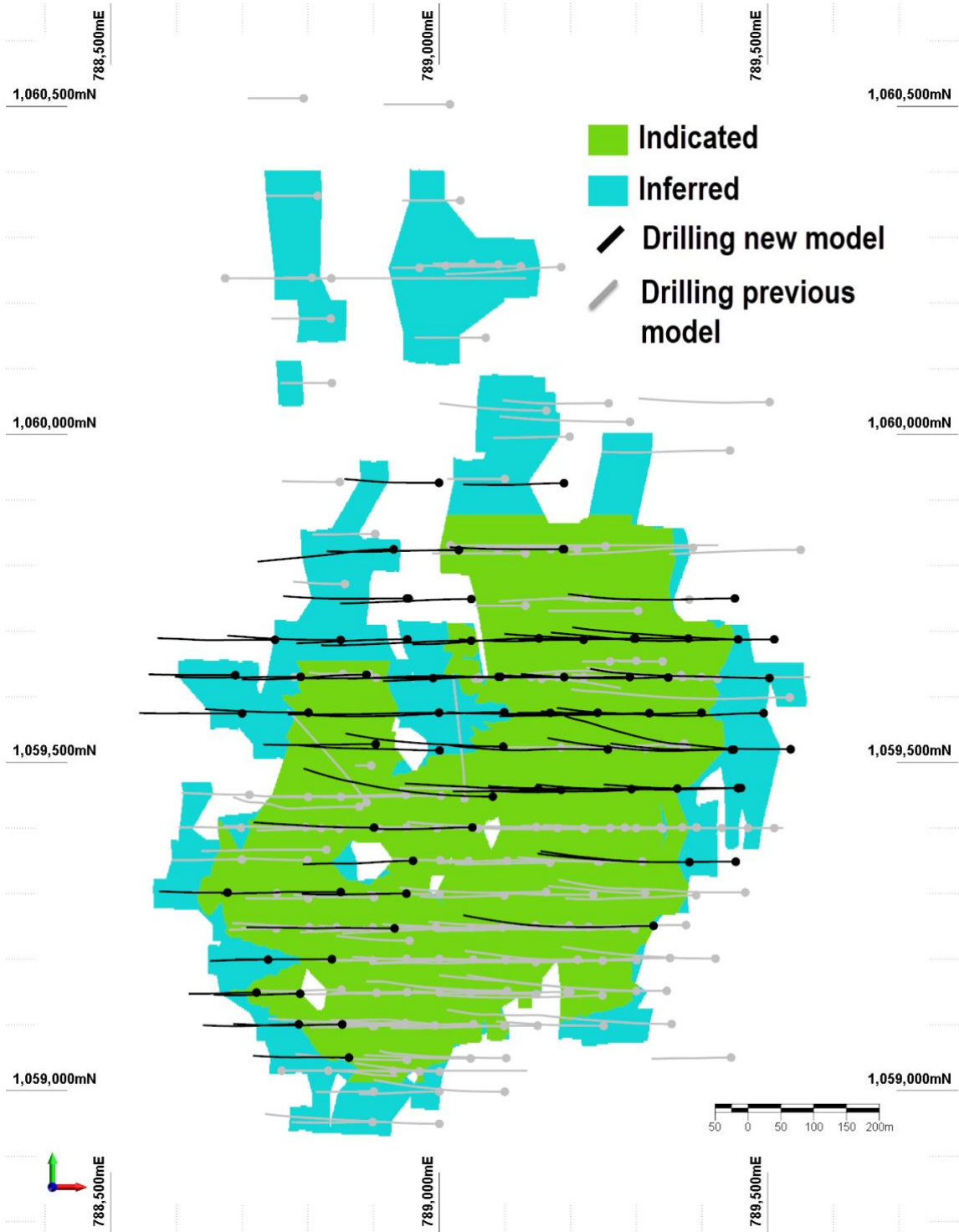
Figure 7: Plan view of BDT2 showing model classification (projected to surface with informing drilling)
