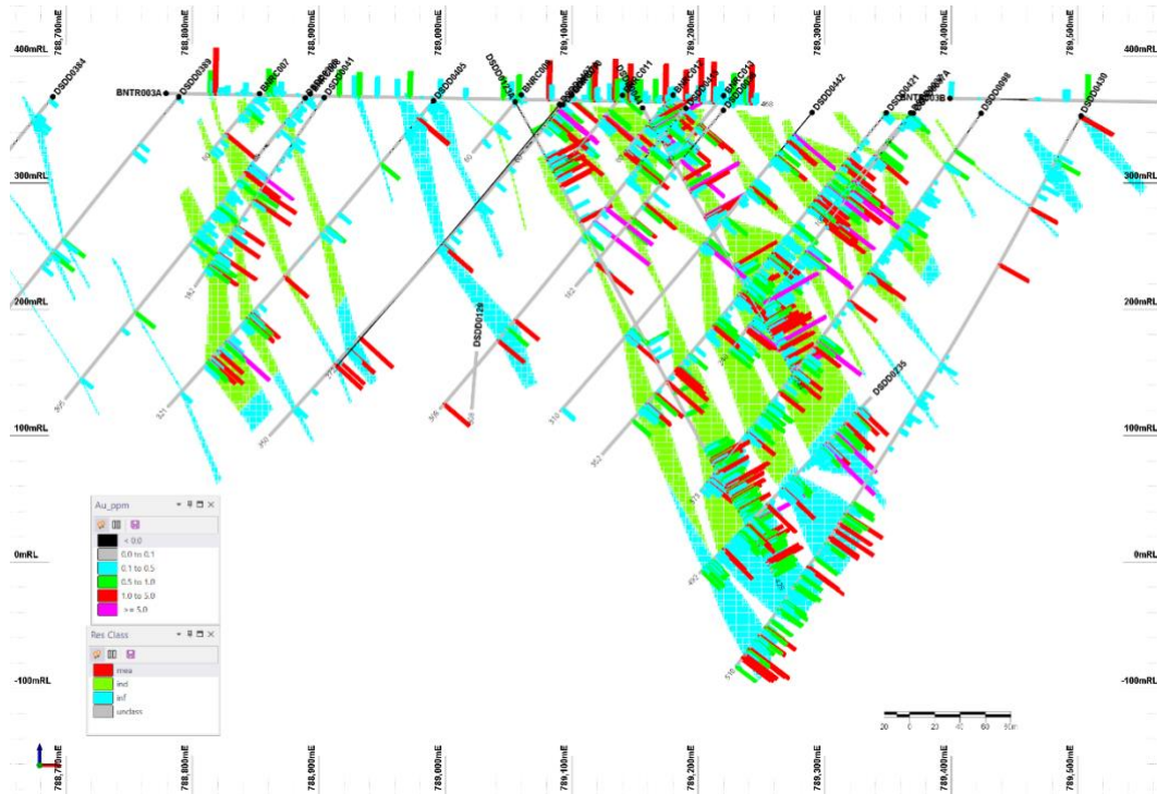
Figure 9: Example cross section (1,059,625mN) BDT2 showing resource classification and drill data (looking north +/-25m)
