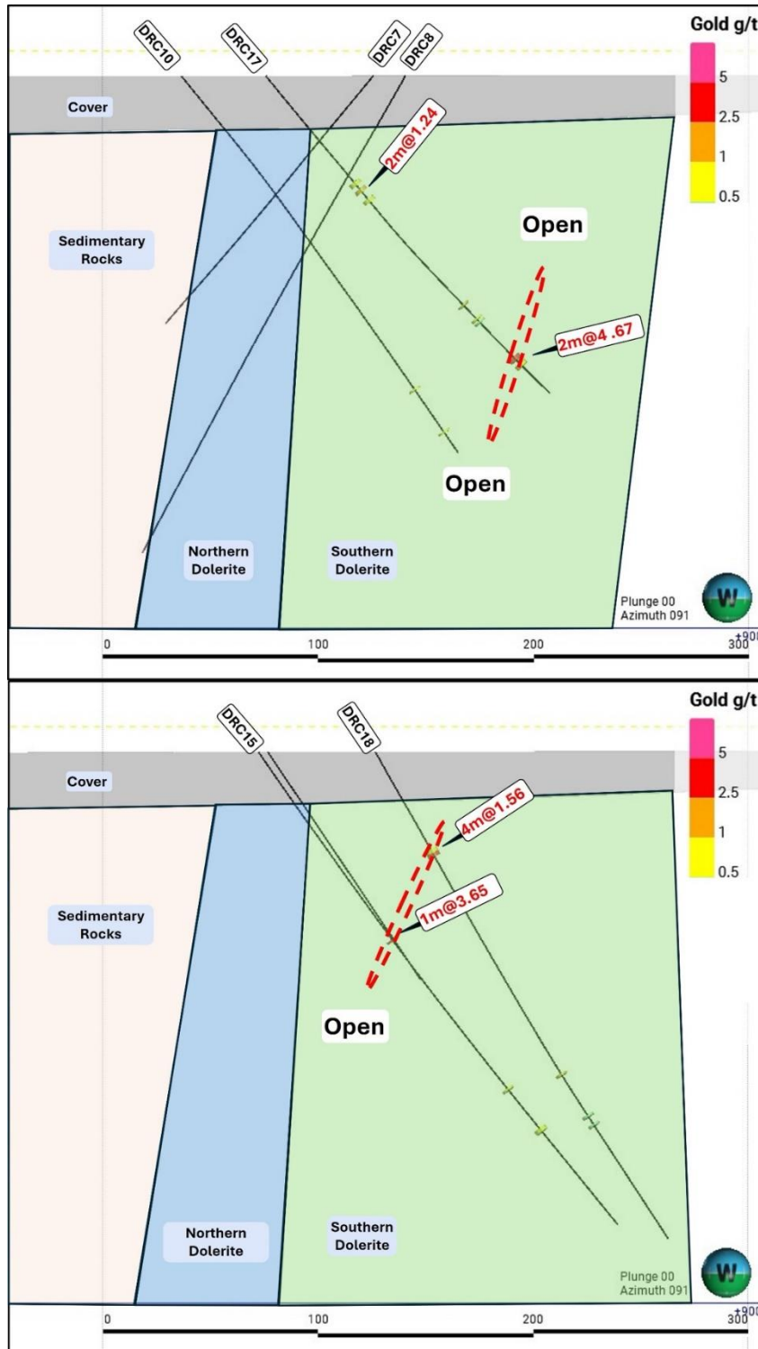
Figure 9: Cross-sections through the Dokwe Central western continuation confirming that gold mineralisation continues beyond the fault that may have terminated the mineralisation.
