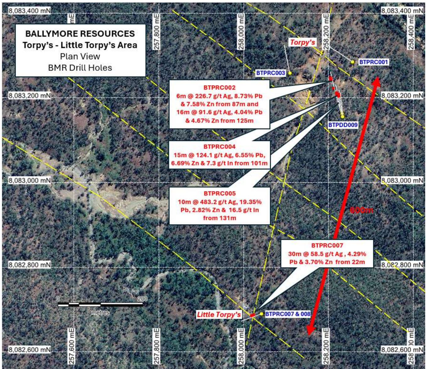
Figure 3 – Airphoto of the Torpy's - Little Torpy's area showing mapped faults (yellow) and Ballymore drill holes with assays.
