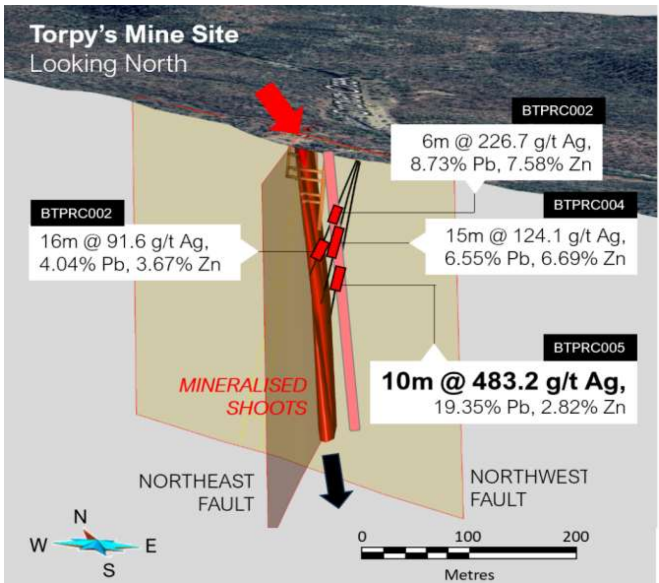
Figure 2 – Oblique section looking north towards the Torpy's prospect showing modelled northwest- and northeast-trending faults and the interpreted mineralised shoots (red) plunging moderately towards the south and the locations of drill holes BTPRC002, 004 and 005.
