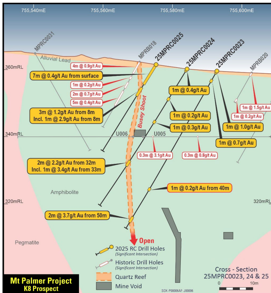
Figure 10. Mt Palmer K8 Prospect Cross Section
