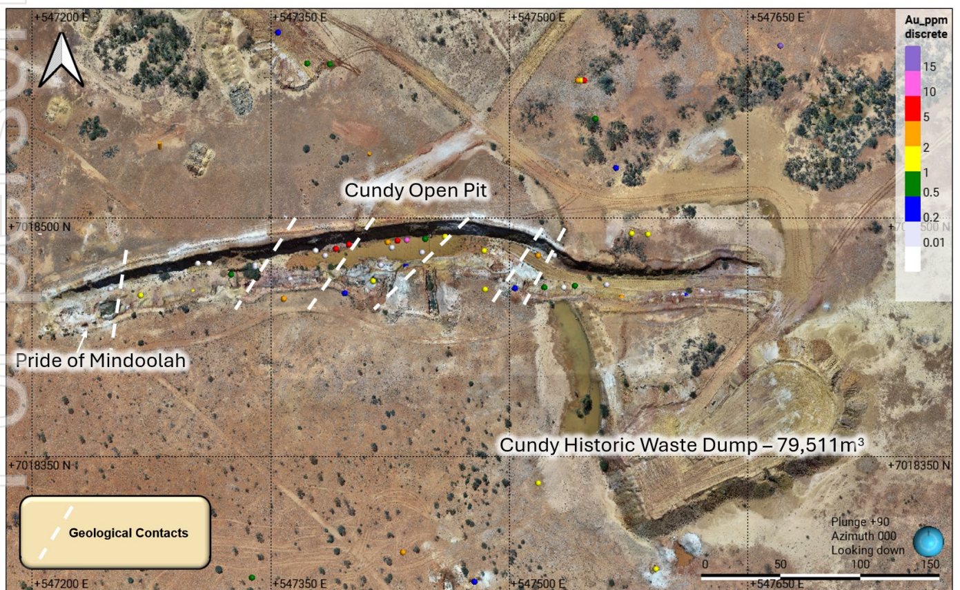
Figure 6. Lidar imagery over of Cundy historic pit and historic waste dump with historic grab samples in plan view (Appendix A – Table 2).
