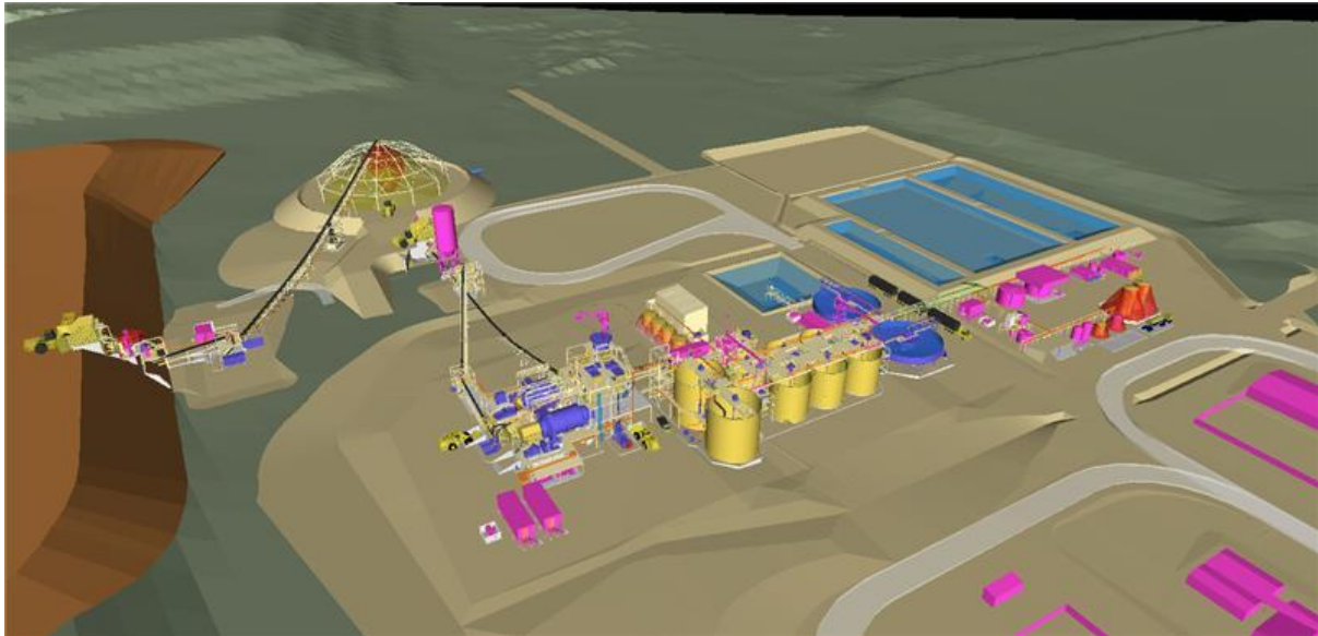
Figure 4: Indicative 3D model of the new 3.0 Mtpa mill
