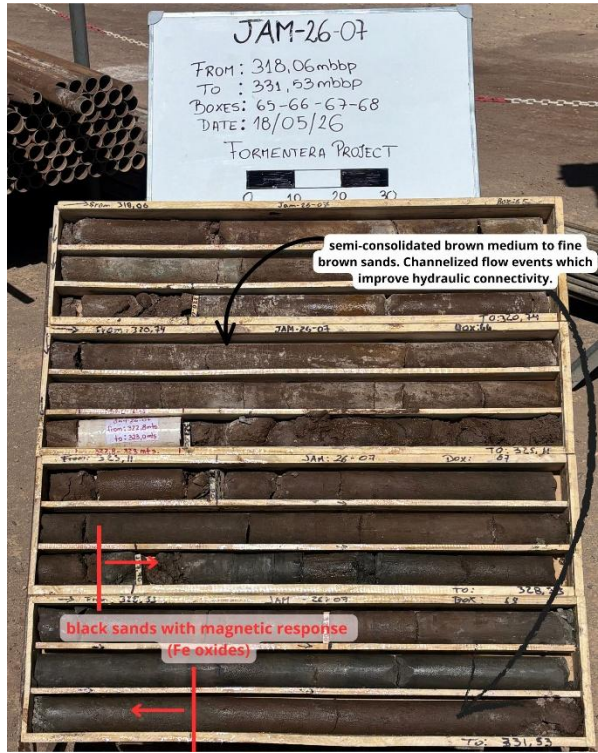
Figure 3. Sections show high porosity and connectivity
