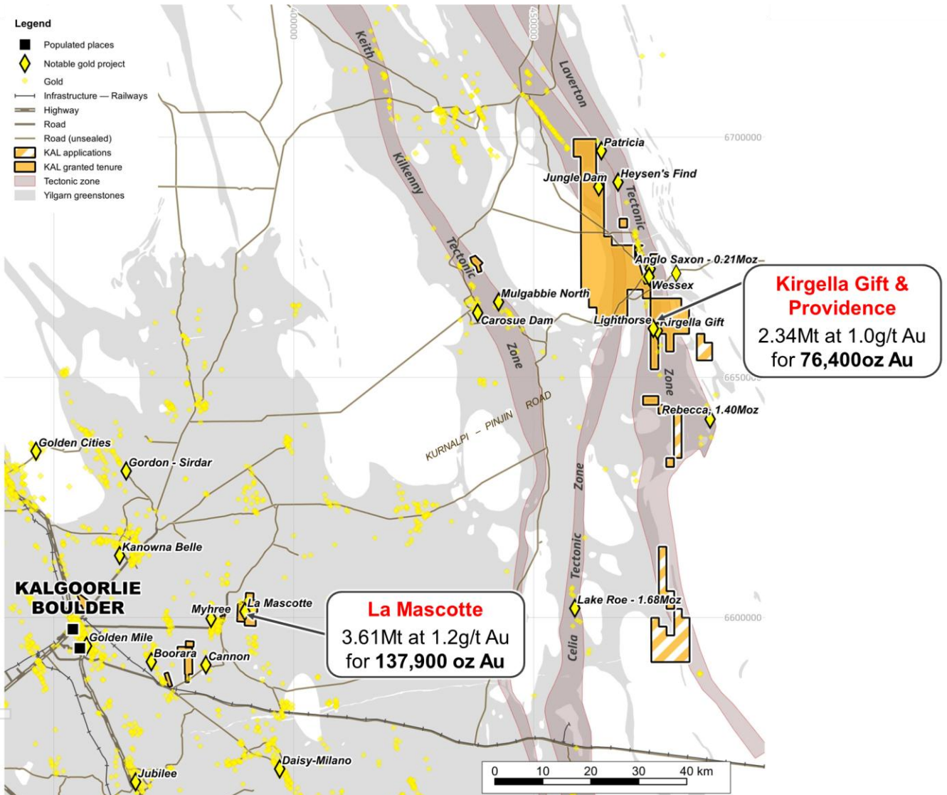
Figure 2 – Location map of the Kirgella Gif-Providence gold deposit and the Lighthorse prospect within KalGold's Pinjin Project, located around 140 km northeast of Kalgoorlie-Boulder. The project is situated approximately 25 km north of Ramelius Resources' (ASX: RMS) Rebecca Gold Project. Also shown is KalGold's outcropping La Mascotte gold deposit 35 km east of Kalgoorlie. Projection: MGA 94 Zone 51.
