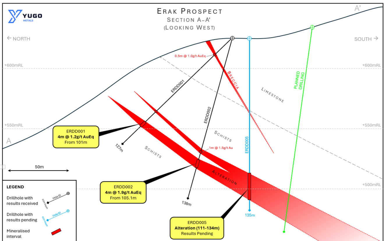
Figure 1: Erak Prospect (Sinjakovo Project), drilling cross-section A-A'
