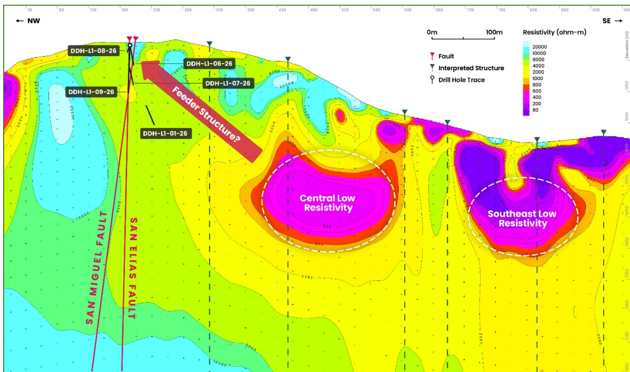
Figure 1: Lirios 1 CSAMT survey, Line 2: 2D inversion model resistivity section with drillholes on ± 15m on section showing the two potential sulphide related resistivity lows and feeder network.
