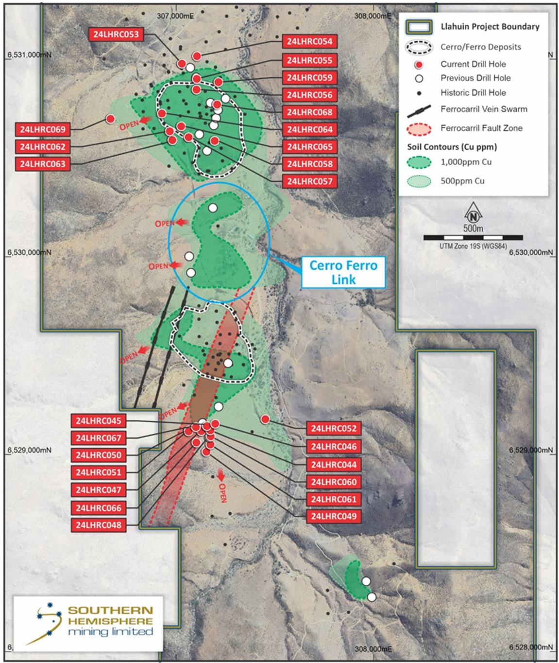
Figure 3: Plan view showing the location of 2024 RC drillholes including 24LHRC055. Holes in white are 2023 drill collars and black are historic.
