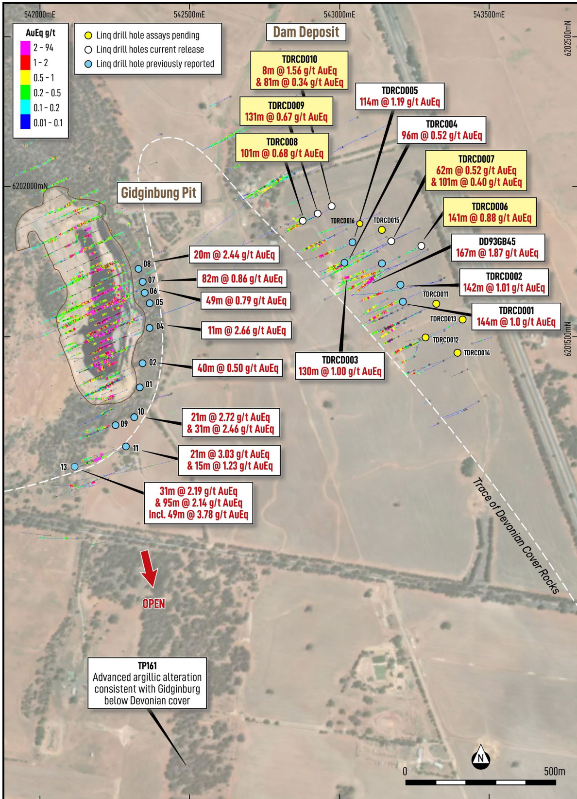
Figure 2: Plan image of Gidginbung and the Dam illustrating the location of drilling results.
