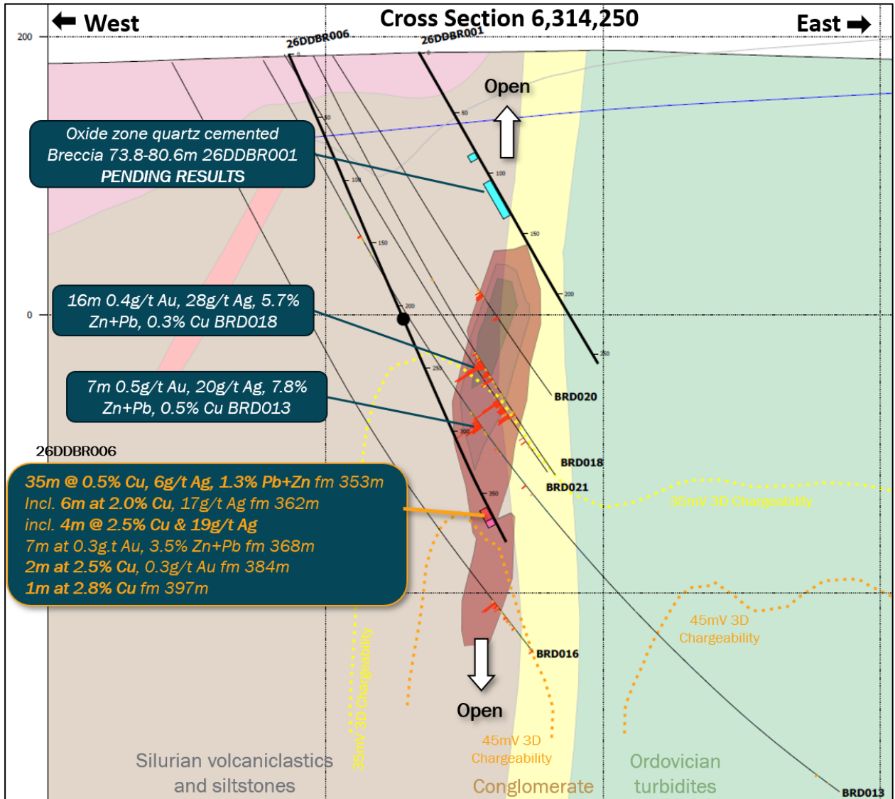
Figure 3: Cross section through 26DDBR006 and 26DDBR001 pending laboratory results (visual results refer ASX AGC 19 May 2026). New results in orange (80m section).
