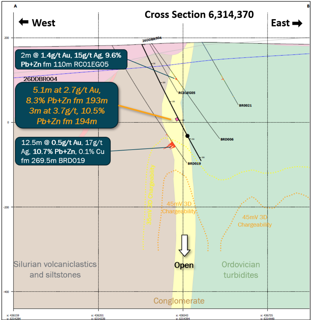
Figure 4: Cross section through 26DDBR004 with new results in orange (50m section).
