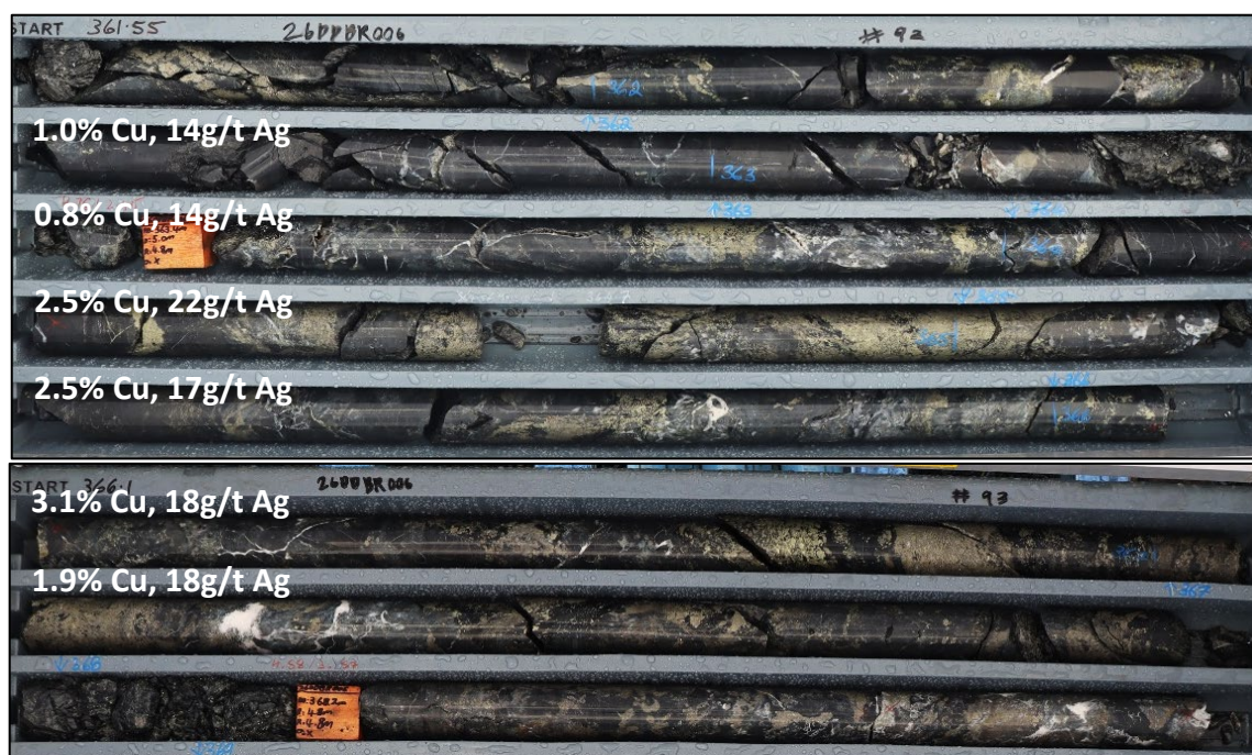
Figure 1: Semi-massive chalcopyrite mineralisation within the 35m mineralised zone intersected in 26DDBR006. The zone in this photo returned 6m at 2.0% Cu & 17g/t Ag from 362m.
