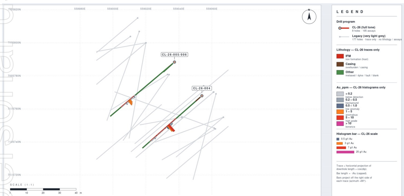
Figure 5. Beaver Prospect Plan View Showing 2026 and Historical Drillholes Traces Within the Mineralised Corridor
