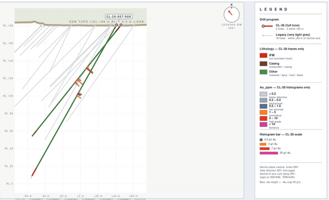
Figure 8. Andrew South Prospect Cross Section - Continuity of the Andrew South Mineralised Corridor
