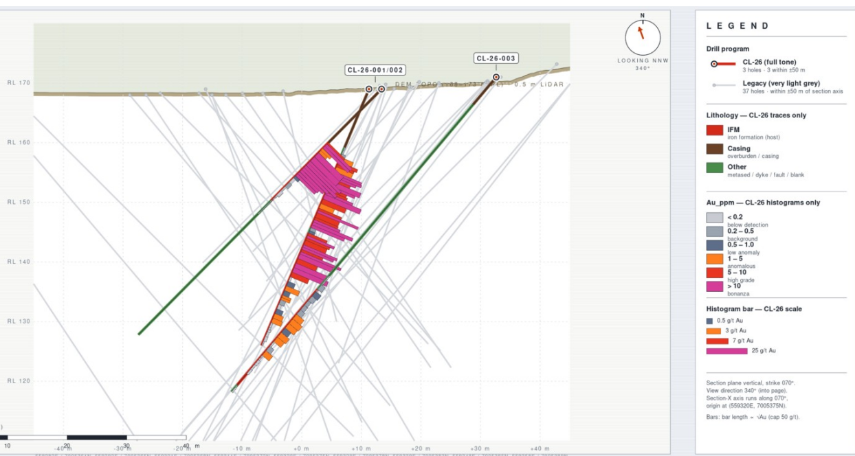
Figure 4. Arrow Prospect Cross Section – Relationship Between Gold Mineralisation, Structure and the Target Horizon Cross section looking northwest through the Arrow Prospect showing CL-26-001, CL-26-002 and CL-26-003 within the Bugow Iron Formation. The section highlights the high-grade mineralisation intersected in CL-26-001 and CL-26-002 and the position of CL-26-003 adjacent to the interpreted mineralised corridor. Combined with downhole IP data, CL-26-003 provides important calibration for the Company's exploration model.
