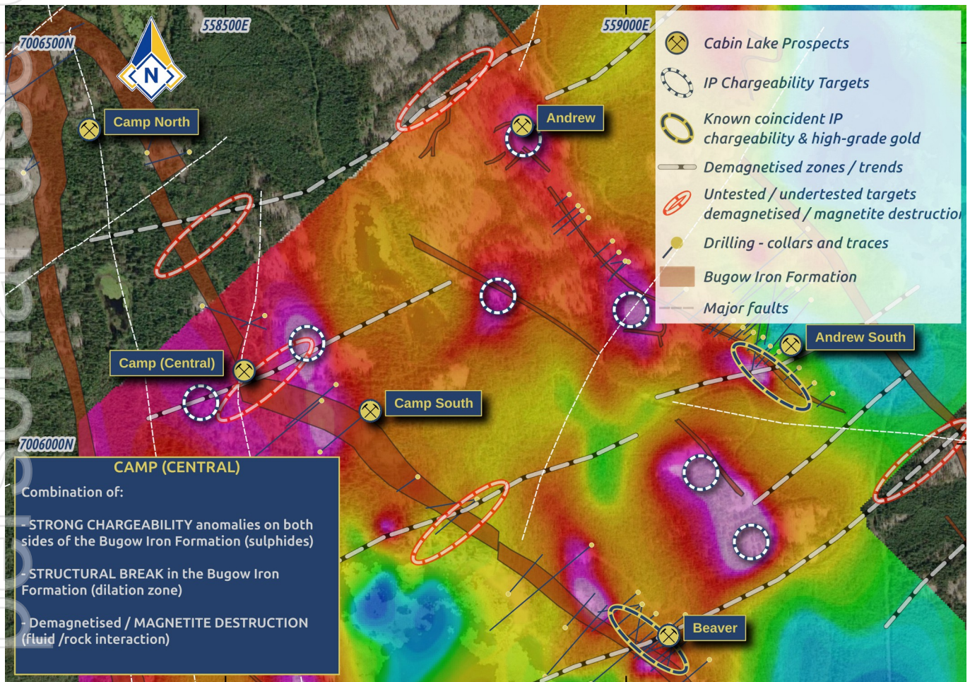
Figure 9. Camp Prospect: Priority Exploration Targets Identified from Integrated IP and Magnetic Surveys
