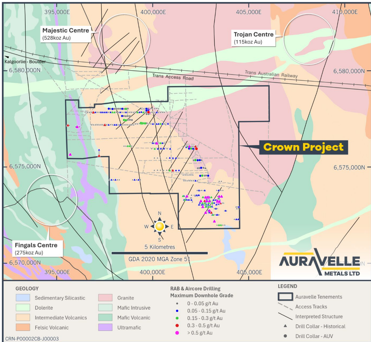
Figure 2: Crown Project - Geology and Drilling 3
