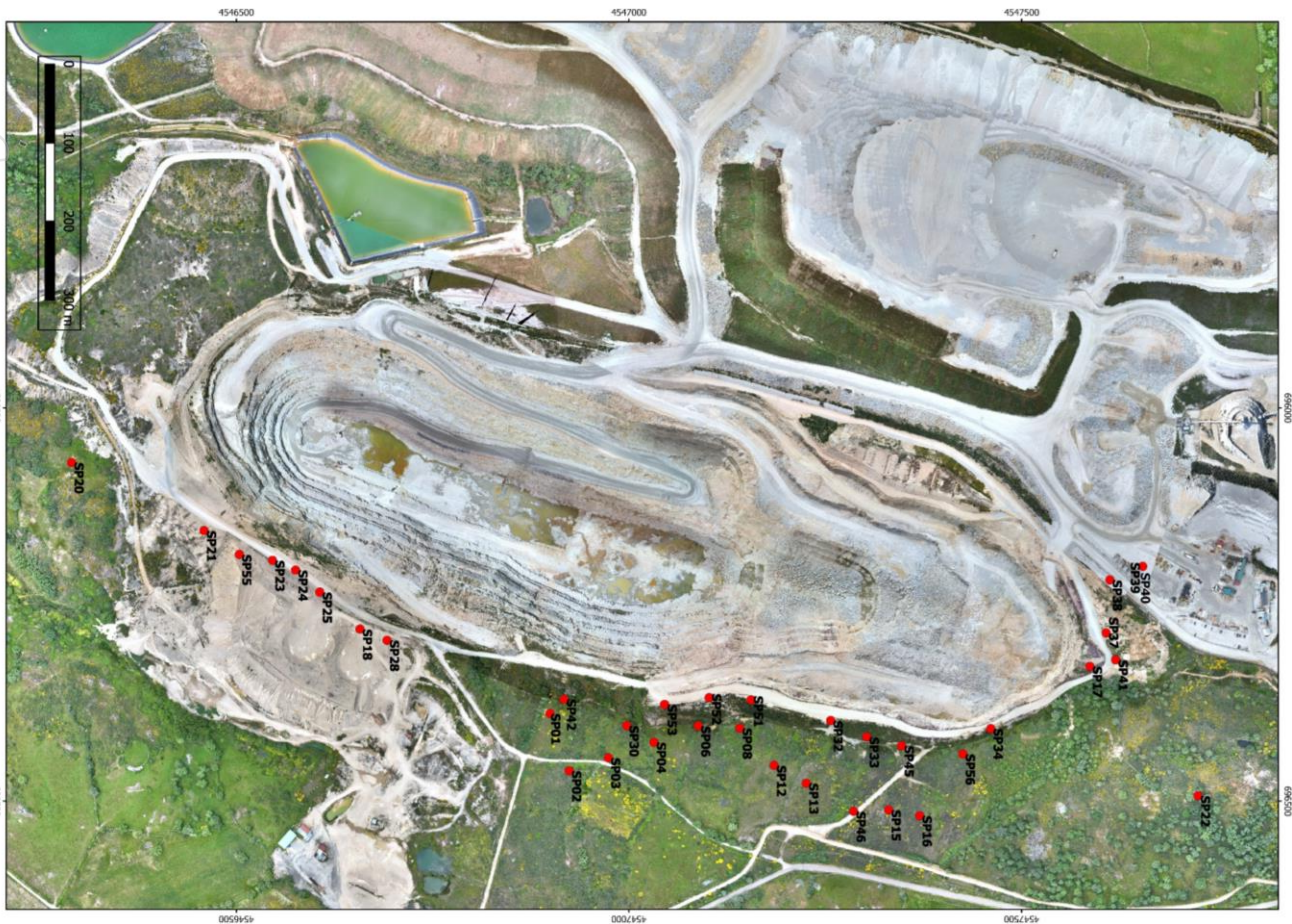
Figure 2: Planned Phase 1 drill hole locations at Barruecopardo
