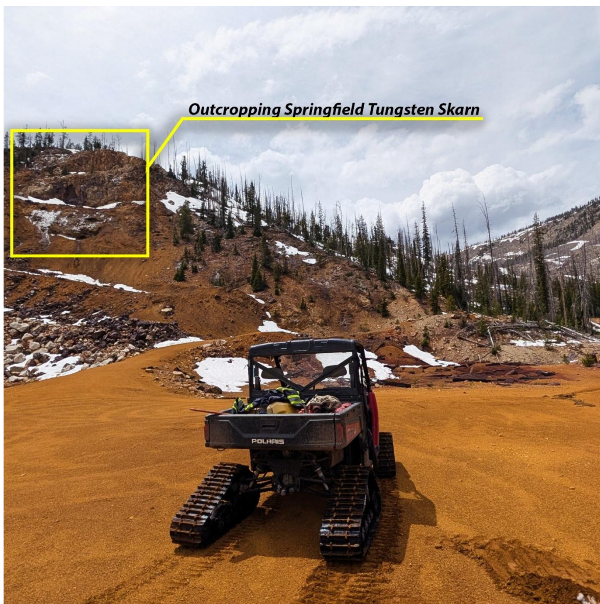
Figure 4: Photo showing the outcropping Springfield tungsten skarn previously mined by Bradley mining Co, high grade tungsten gold and gallium rock chip sample results shown in figure are taken from the outcrop shown and surrounding areas.
