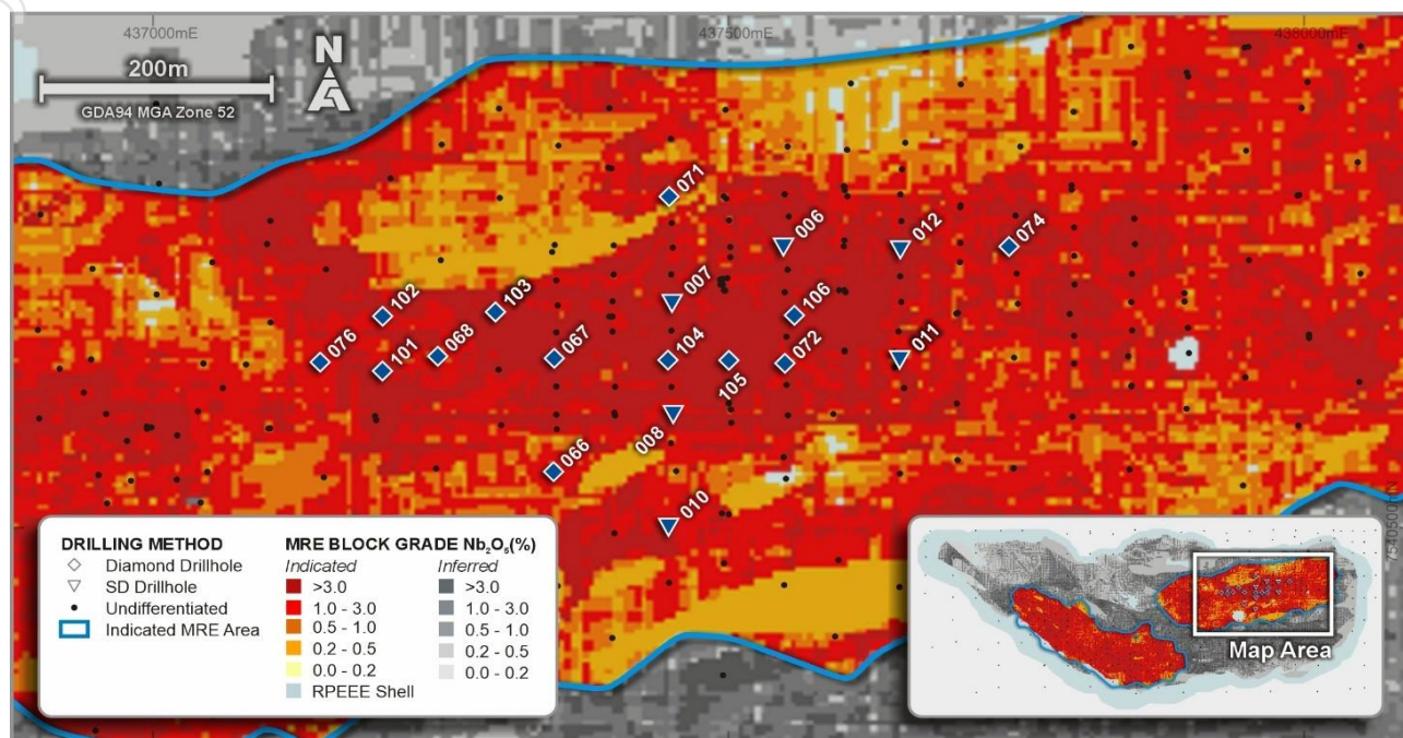
Figure 3: Location of Composite A drillholes
