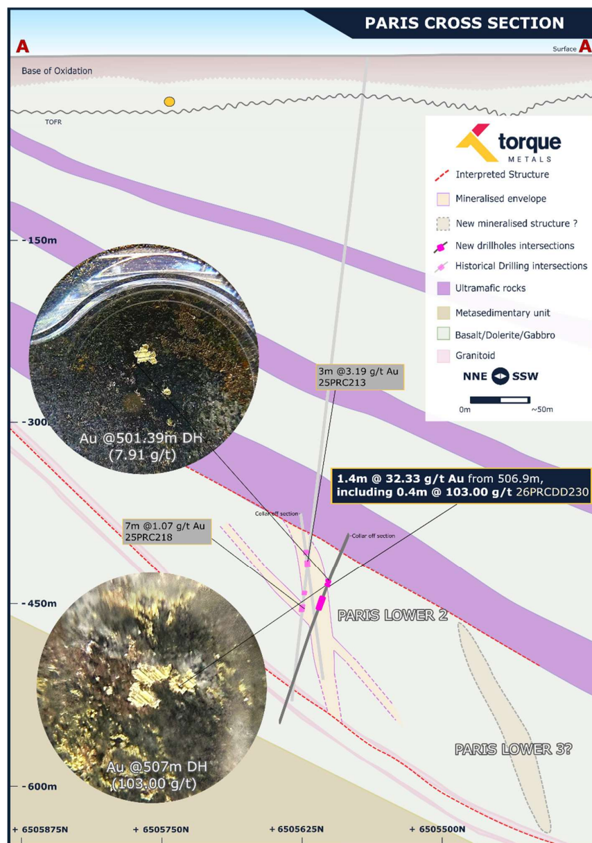
Figure 2: Paris Gold Deposit cross section, highlighting the multi lode system and recent intersections. Visible gold shown above is from hole PRCD230 and has been assayed, the results of which are reported in this release
