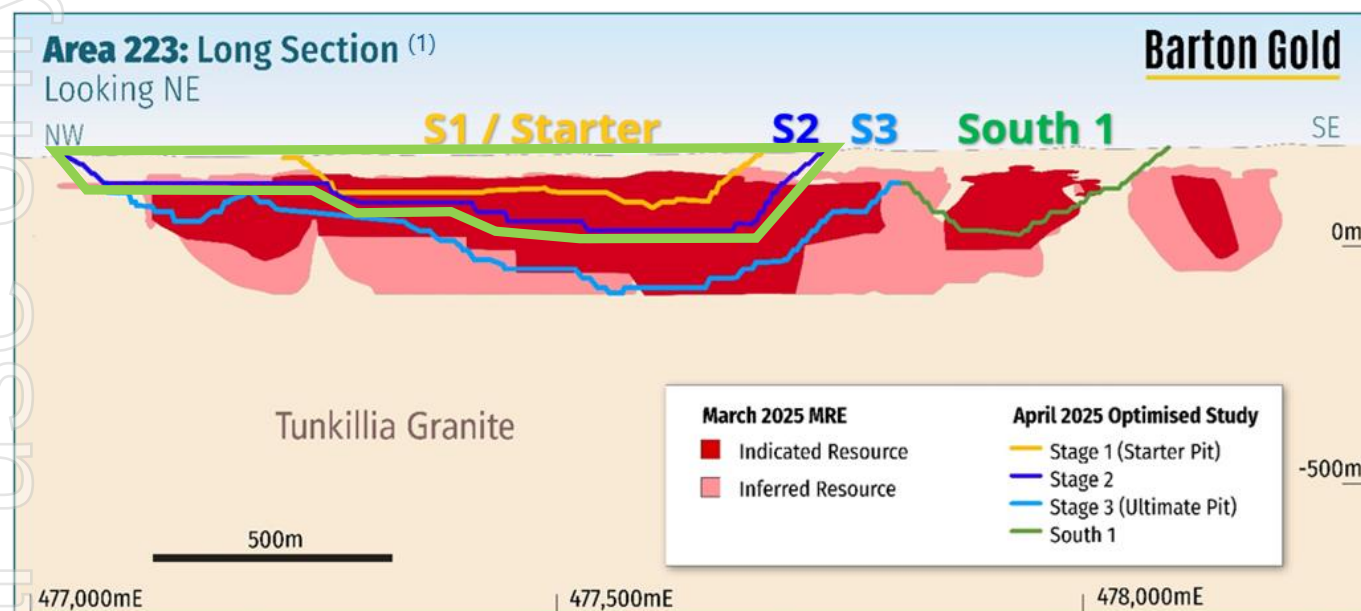
Fig. 2 – Location of 2025 Phase 1 RC upgrade drilling (green polygon) on main optimised open pit 7
