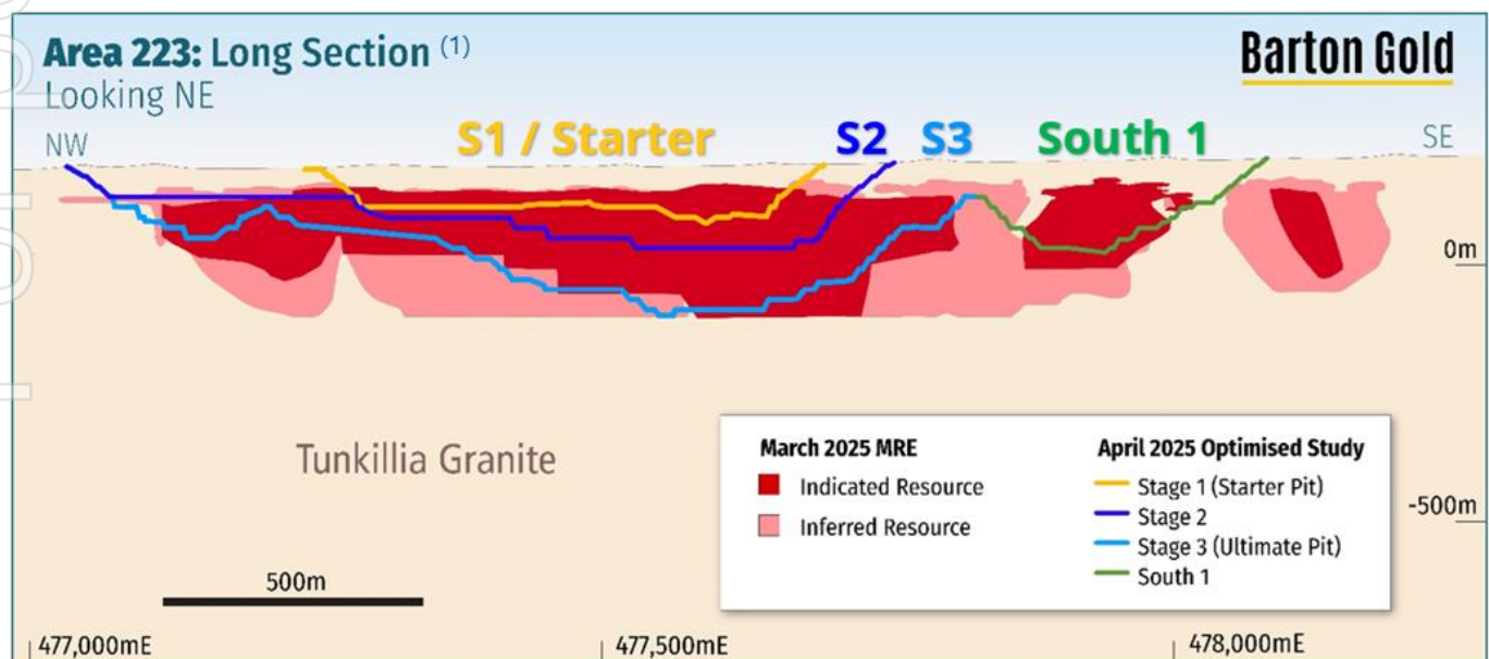
Fig. 1 – Tunkillia 'Area 223' optimised open pit long section showing high value S1 / S2 pit zones 4
