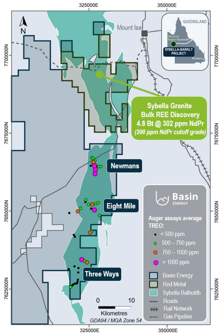
Figure 4 – Granite anomalies identified in 2023 Auger Sampling 4,5 .
