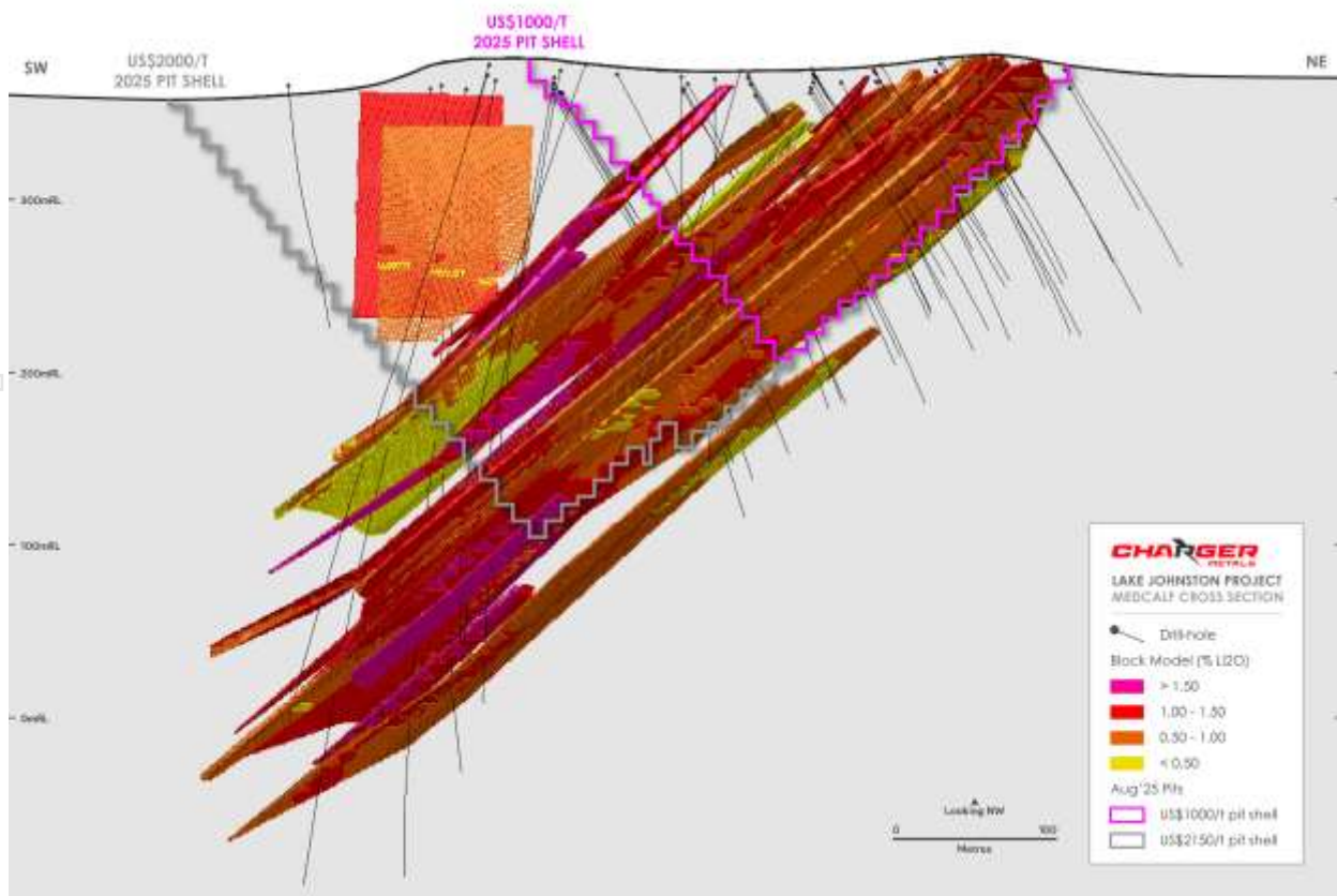
Figure 2. Oblique sectional view of the Medcalf Lithium Mineral Resource showing the 2025 pit optimisations based on SC6 US$1,000/t and US$2,000/t.
