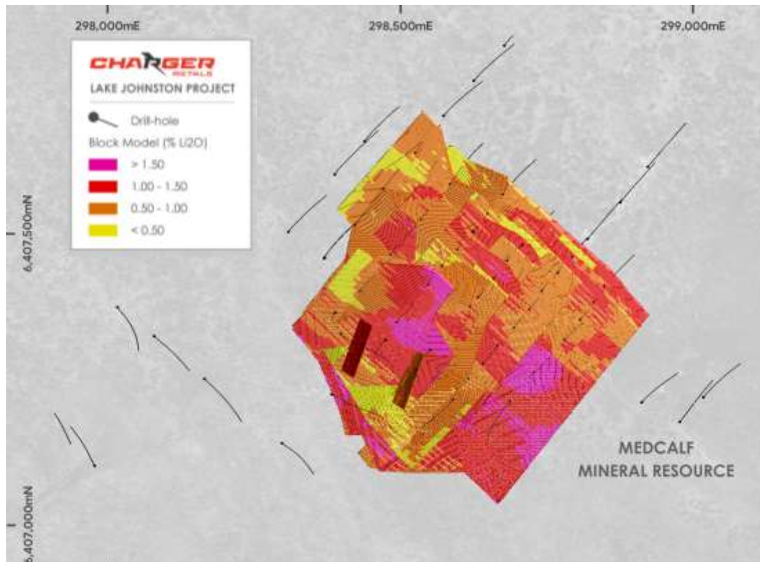
Figure 3. Plan view of the Medcalf 10.6Mt Lithium MRE.
