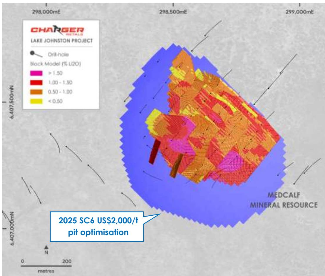
Figure 4. Plan of the Medcalf 10.6Mt Lithium MRE with the 2025 SC6 US$2,000/t pit optimisation.
