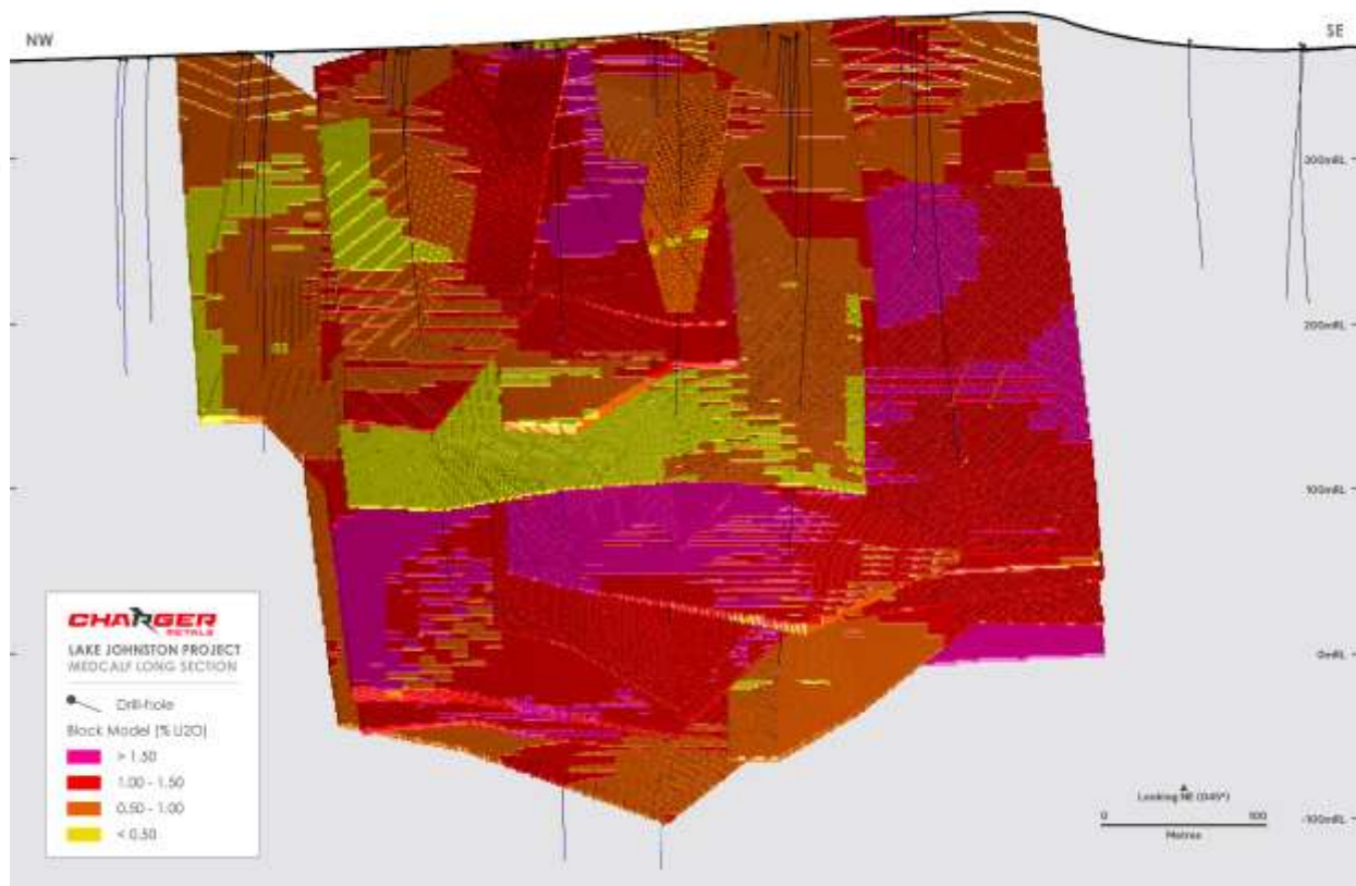
Figure 1. Long sectional view looking northeast of the Medcalf Lithium Mineral Resource.
