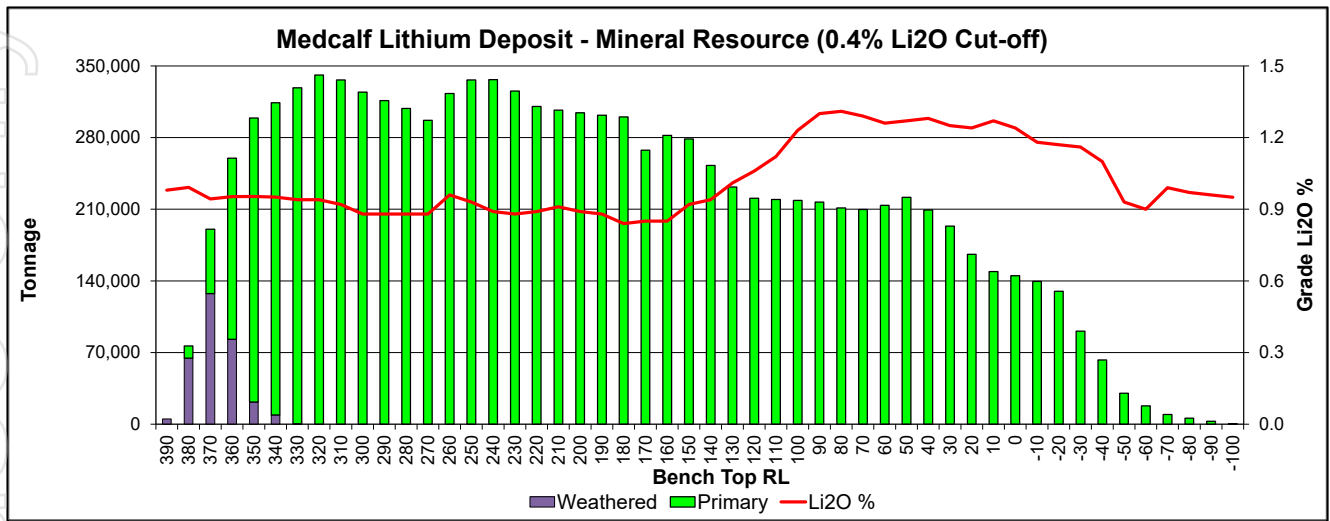
Figure 5 Medcalf Tonnage and Grade – 10m Bench Elevation
