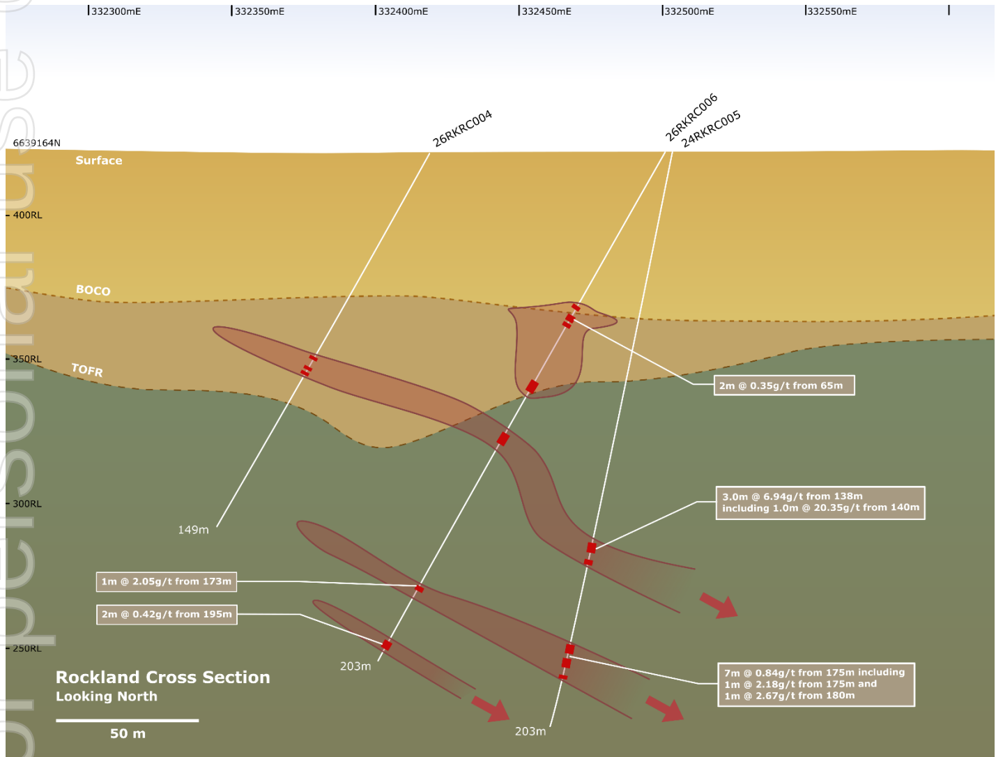
Figure 4: Interpretive cross section of drill line 6639164N
