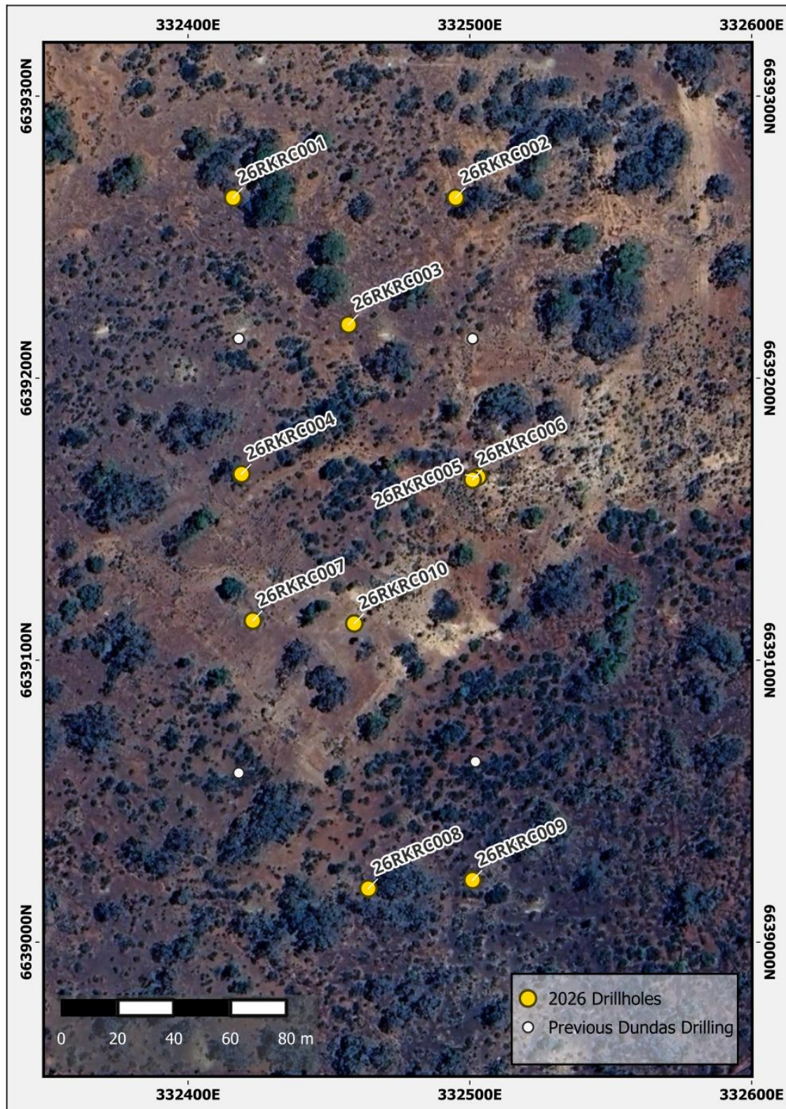
Figure 6: Plan view of Rockland showing drill collar locations (note: Hole 5 and 6 were drilled vertical and 60 degrees to the West respectively from essentially the same collar)
