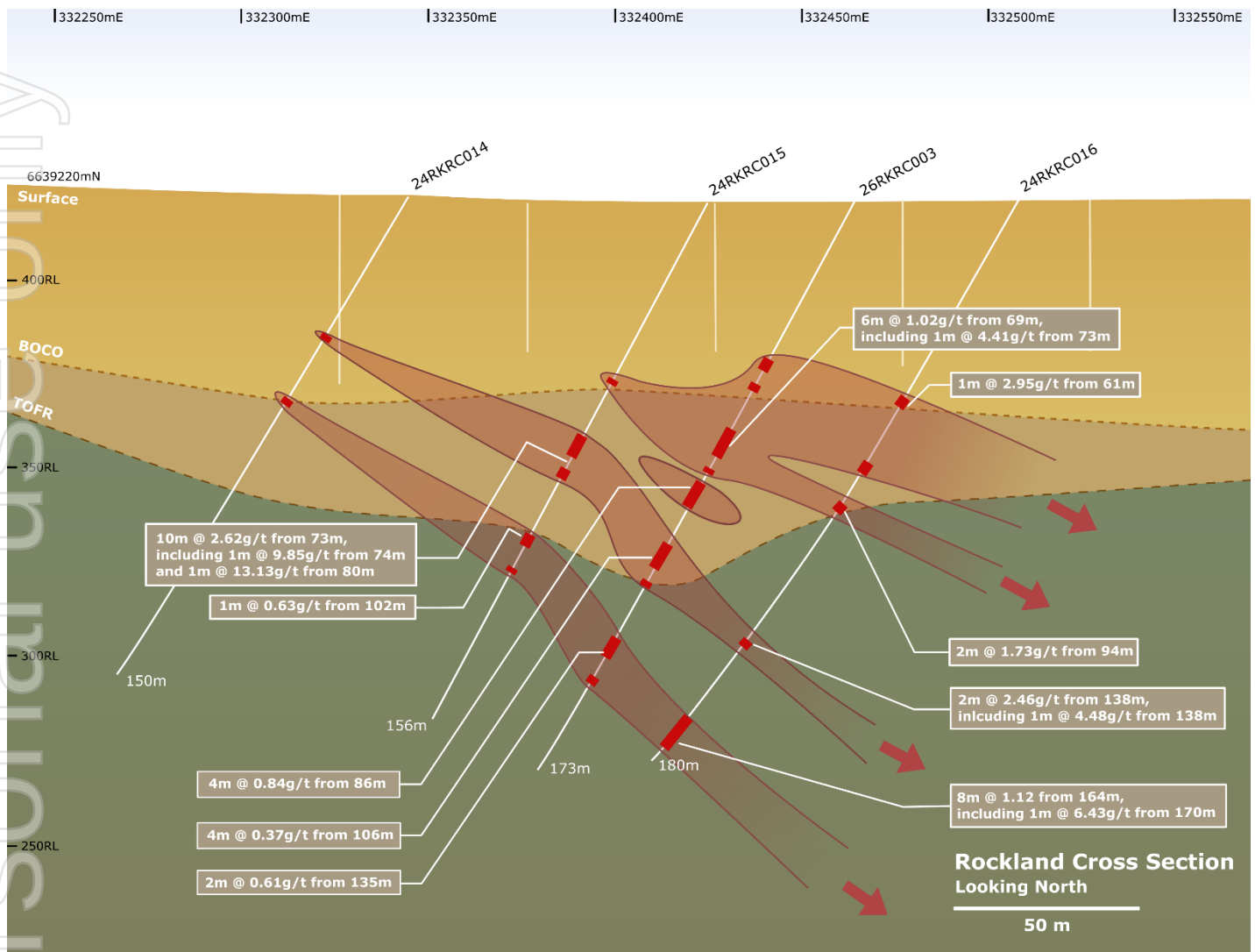
Figure 5: Interpretive cross section of drill line 6639220N
