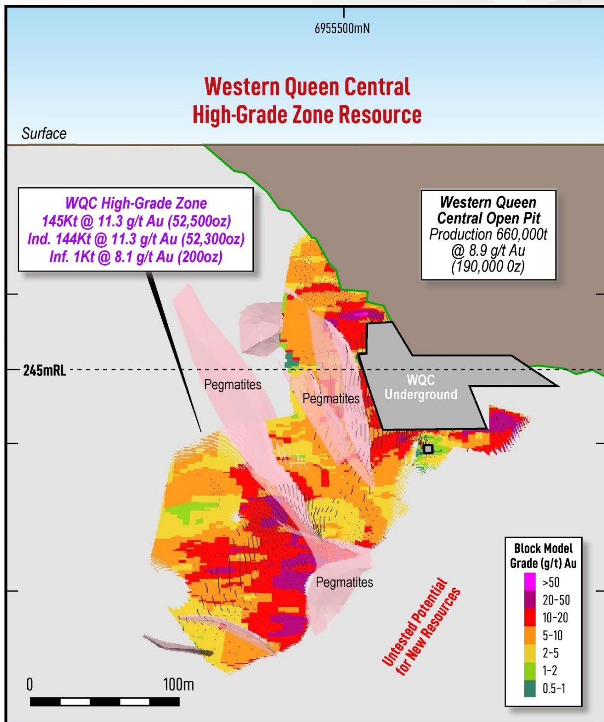
Figure 3 – Newly defined high-grade gold zone below the Western Queen Central pit and underground workings
