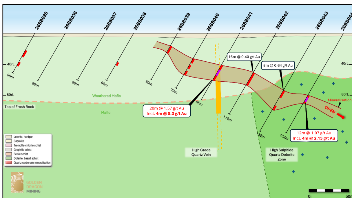
Figure 2. Drill Cross Section 69957750mN highlighting moderately east-dipping gold lode within the upper portion of an altered, pyritic dolerite and the newly identified northeast trending high grade quartz veins.
