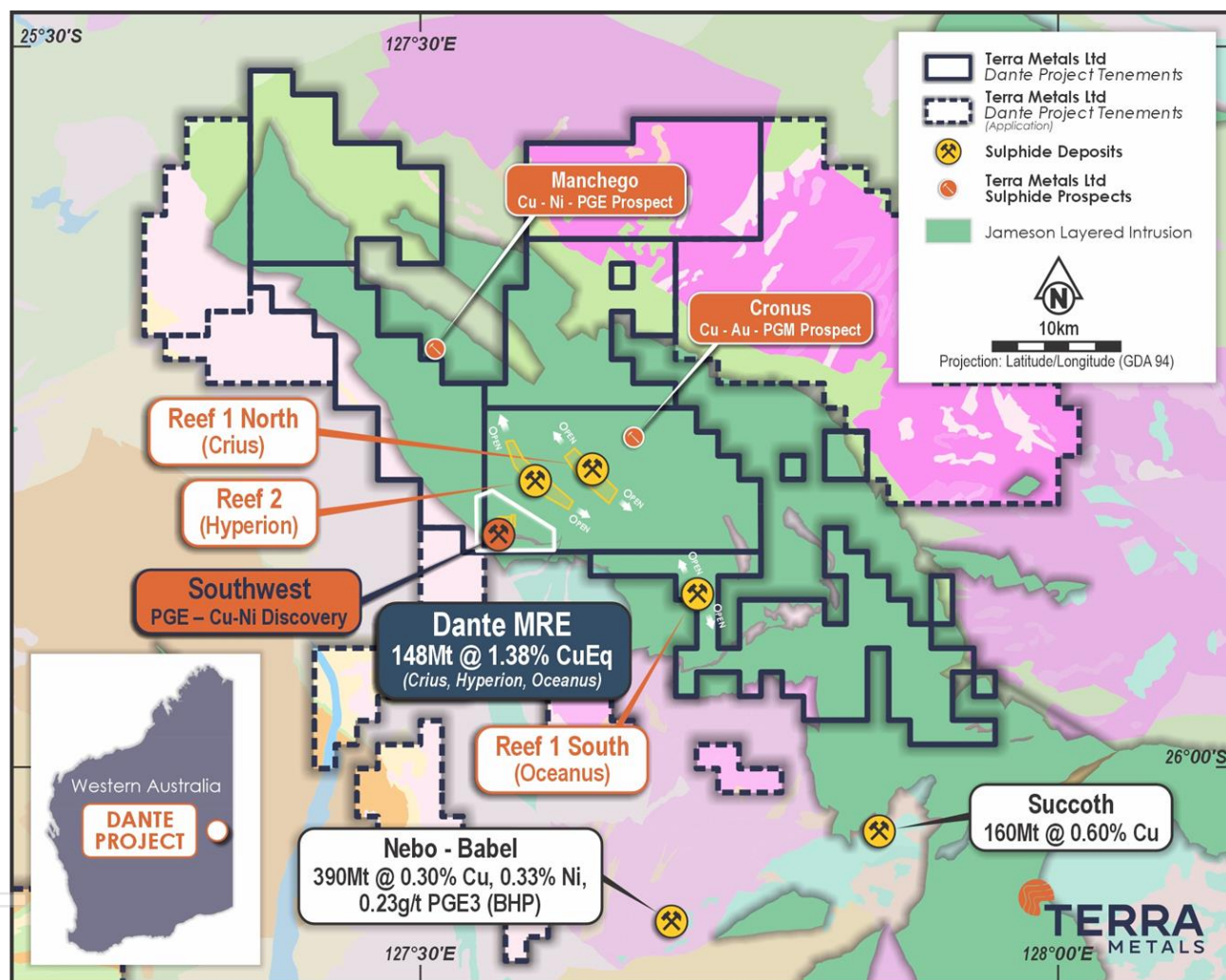
Figure 1. Location of the Company's Dante Project tenure, overlying the geology map of the West Musgrave Region.
