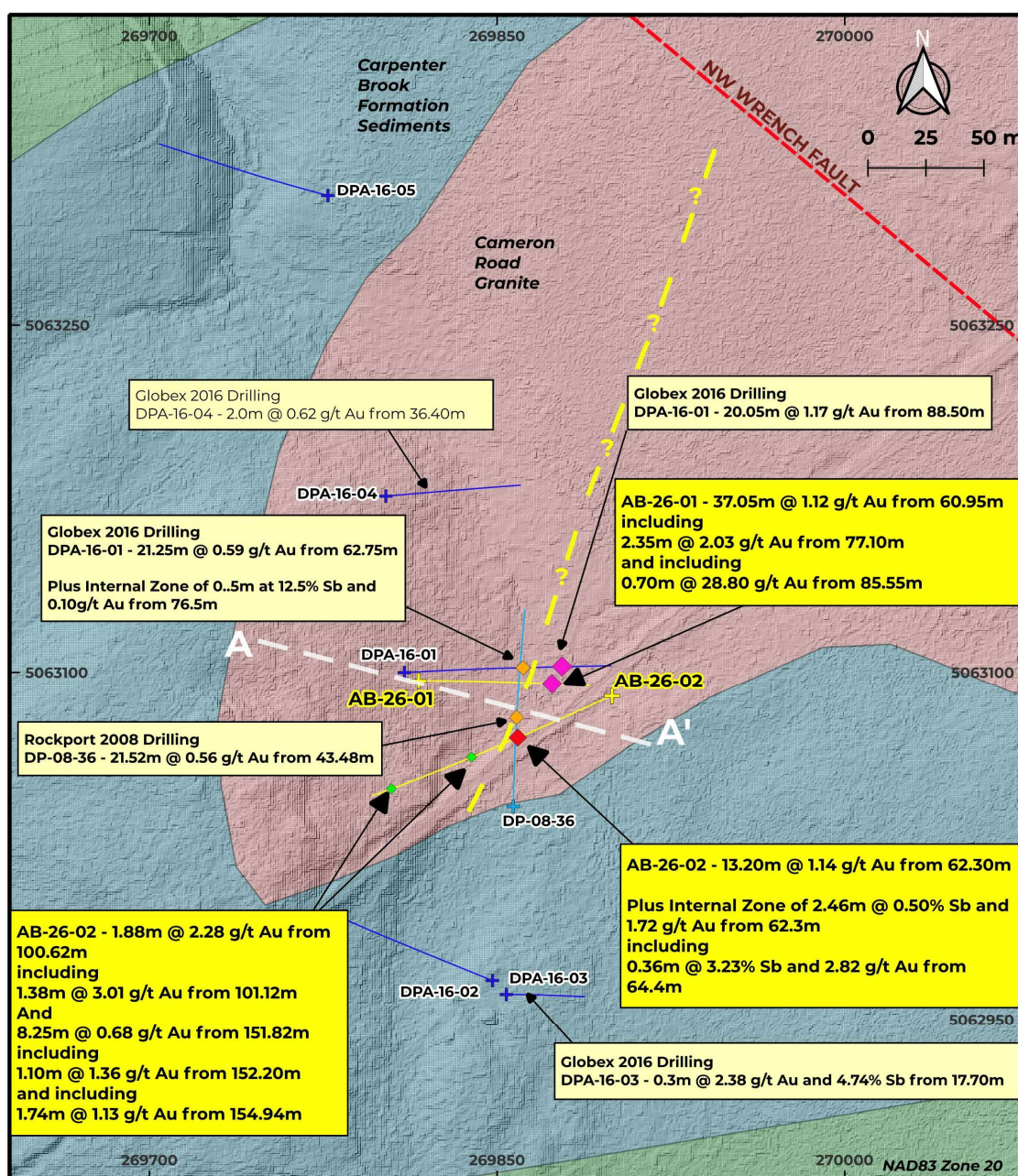
Figure 2: Collar Plan Albright Brook Prospect
