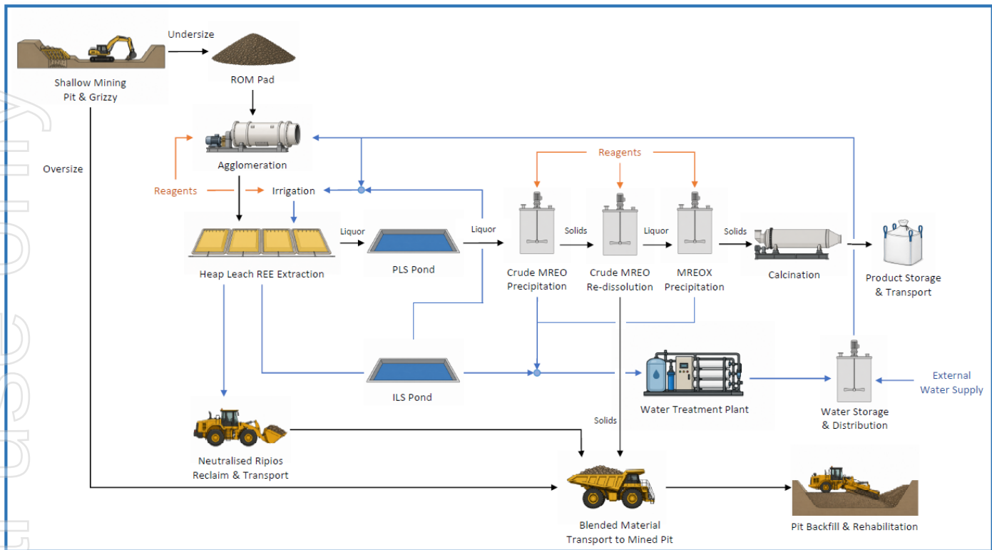
Figure 4 Koppamurra Flowsheet
