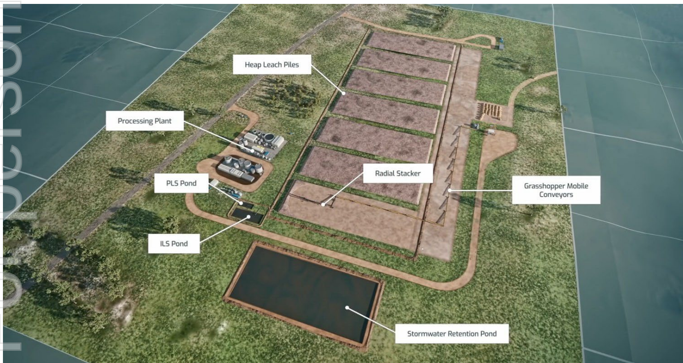
Figure 5 Birdseye view of the processing plant model
