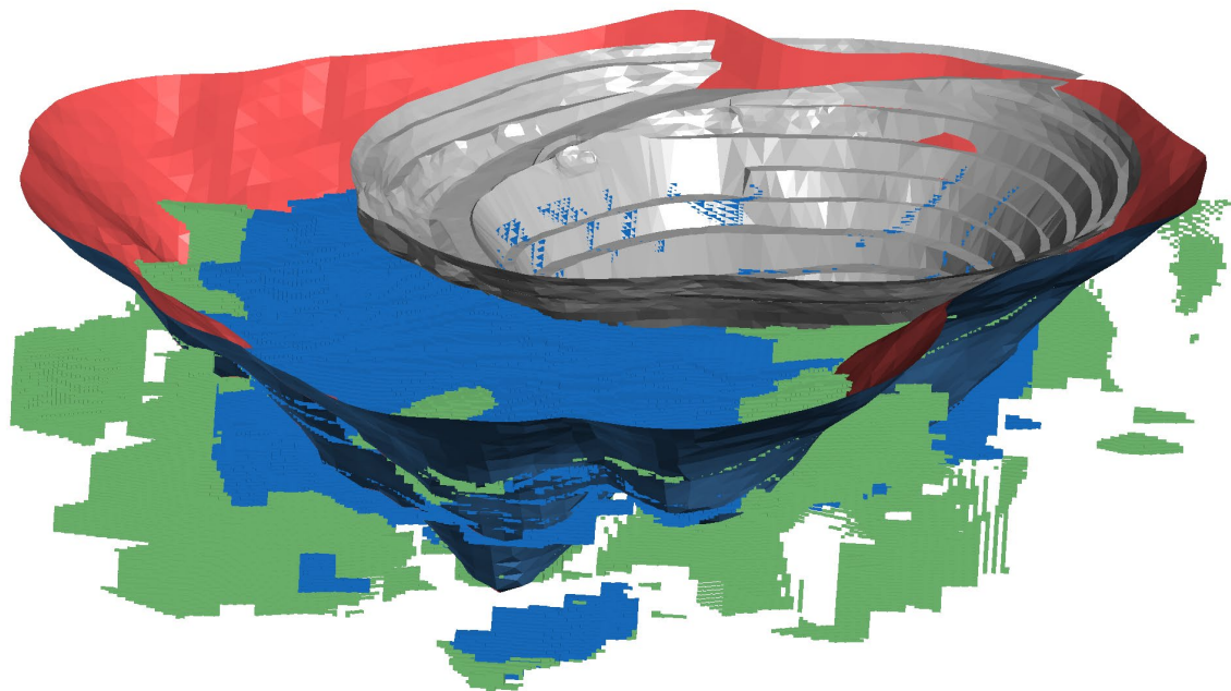
Figure 5: Oblique image looking NE showing Resource classification (blue=Indicated, green=Inferred) for Imperial. Historically mined pit (grey) and AS6,000oz optimized pit shell (red/blue)
