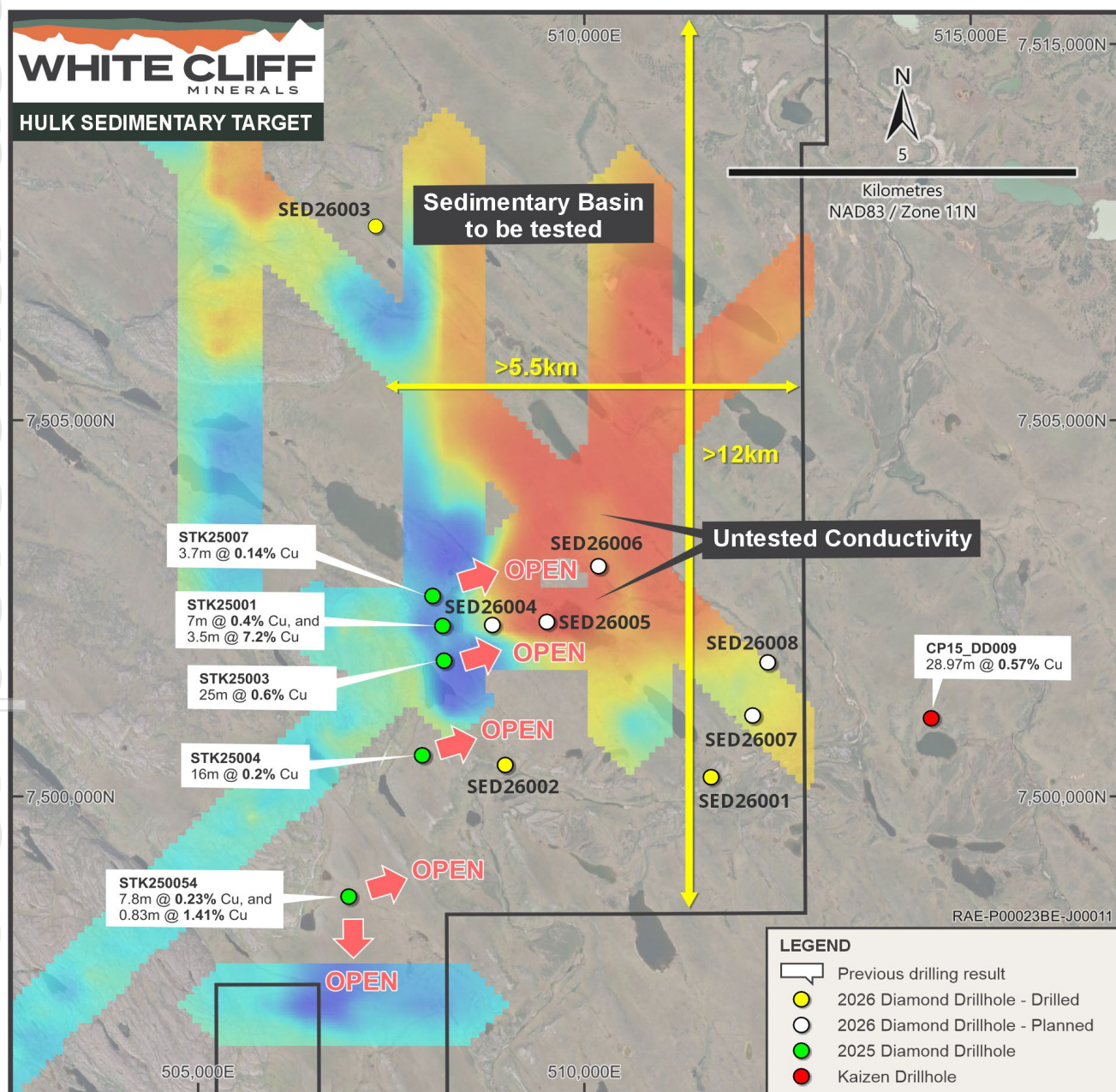
Figure 1 - Map of 2026 diamond drillholes depicting the regional scale of drilling which has returned copper mineralisation at the base of the Rae Group.
