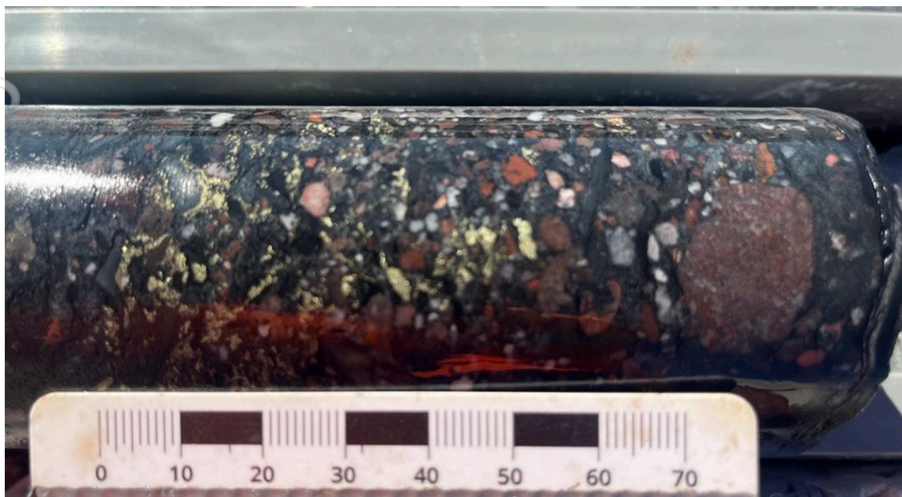
Figure 2 – Photograph of chalcopyrite forming a cement phase of the conglomerate unit at the contact between the Rae Group and the underlying Husky Creek Formation within hole SED26001. (238.4-238.52m)
