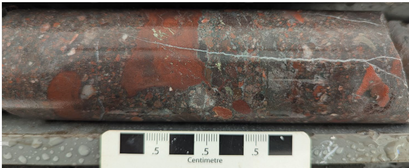
Figure 3 - Photograph of disseminated, fine grained chalcopyrite within the basal conglomerate at the contact of the Rae Group and underlying Husky Creek Formation in drillhole SED26002. (207.1-207.5m)
