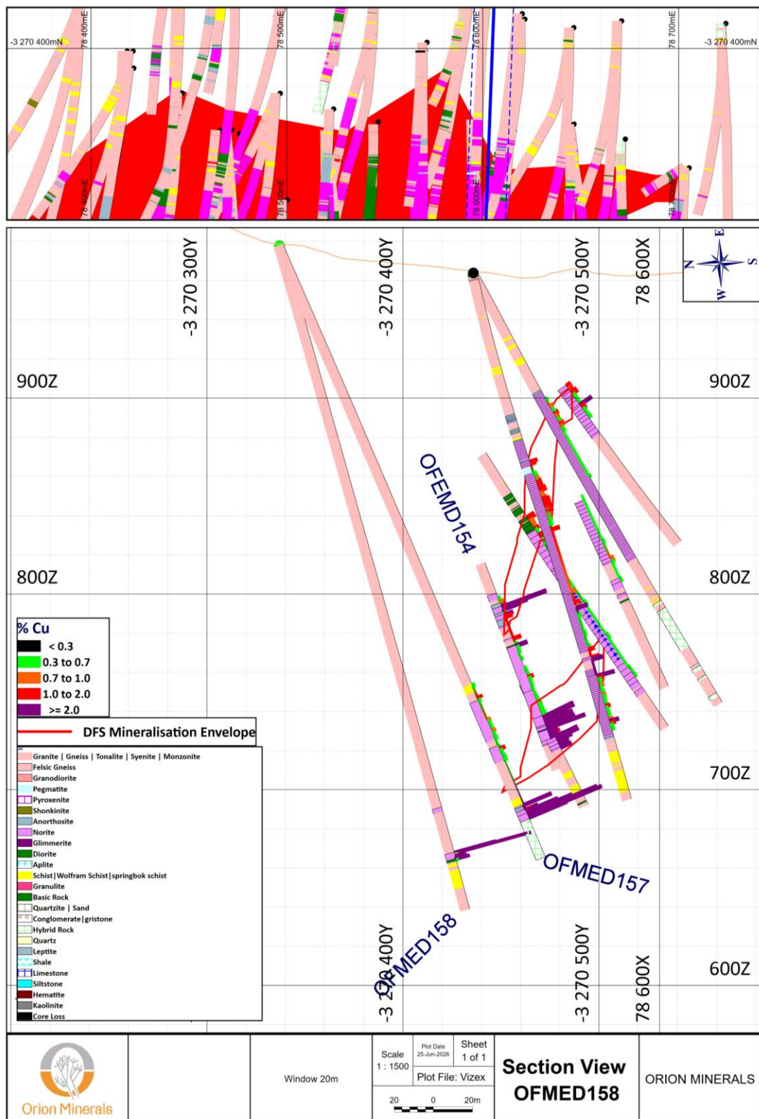
Figure 2: Cross-section of OFMED158 with assay results plotted, with adjacent holes. Mineralisation model not yet updated to incorporate new drill hole intersections.
