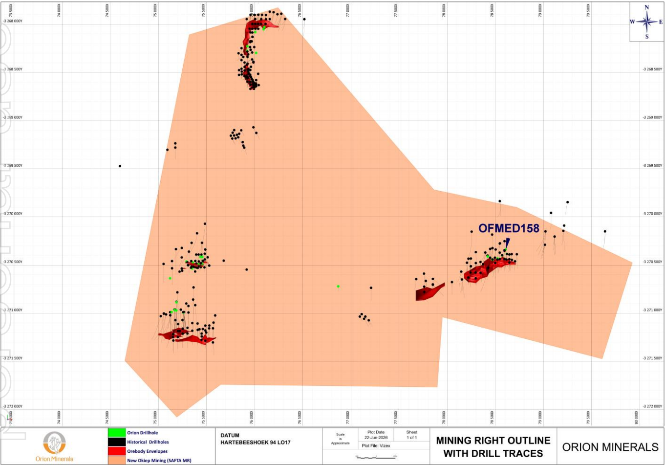
Figure 1: Plan showing historical and Orion (green-labelled) drill holes, including OFMED158 at Flat Mine East, interpreted mineralisation envelopes and extent of the Mining Right.
