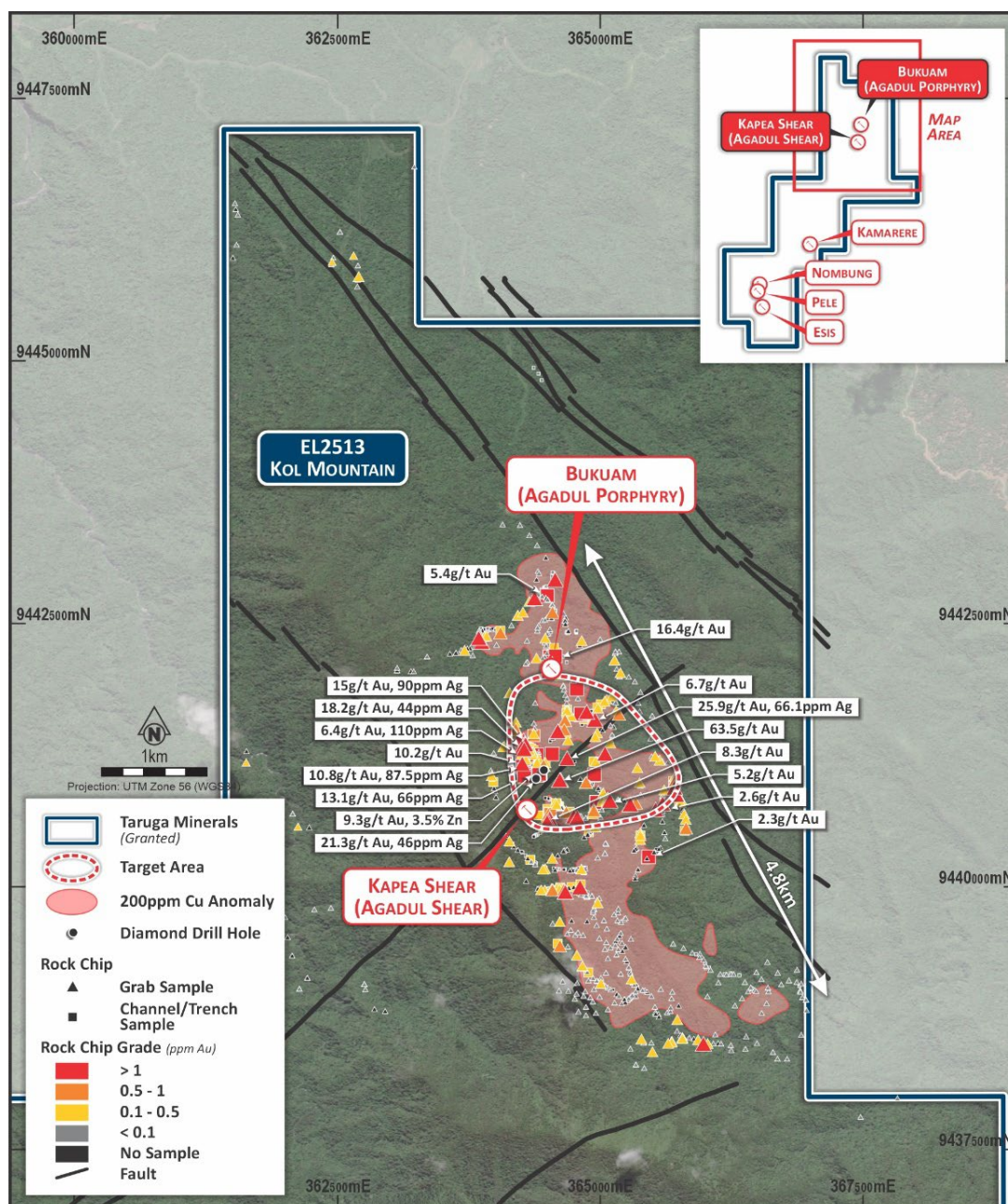
Figure 5: Agadul Prospect, northern Kol Mountain, showing the high priority target area with gold in rock chip results over the 4.8km long 200ppm copper in soil anomaly.
