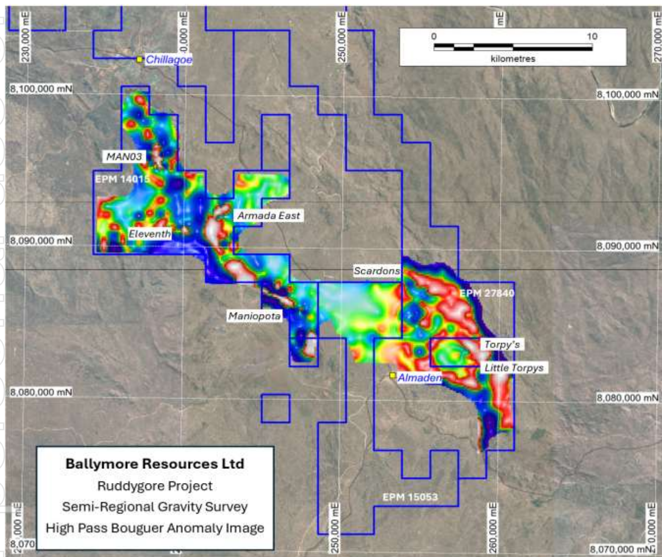
Figure 1 – Ruddygore gravity high pass filter Bouguer anomaly image based on preliminary gridded data.
