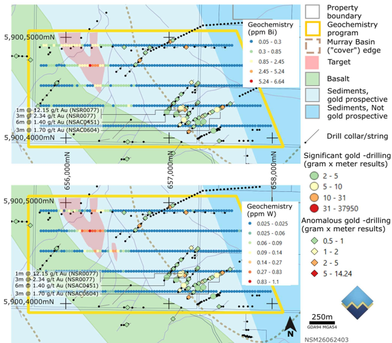
Figure 3 Bismuth and Tungsten geochemistry, Caledonia Prospect.
