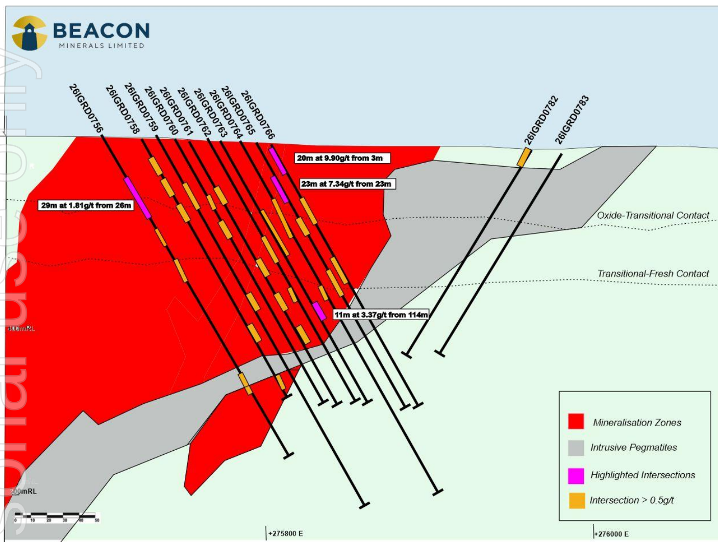
Figure 4: Cross Section of Iguana Resource Development Drill Program 662,3900 Northing
