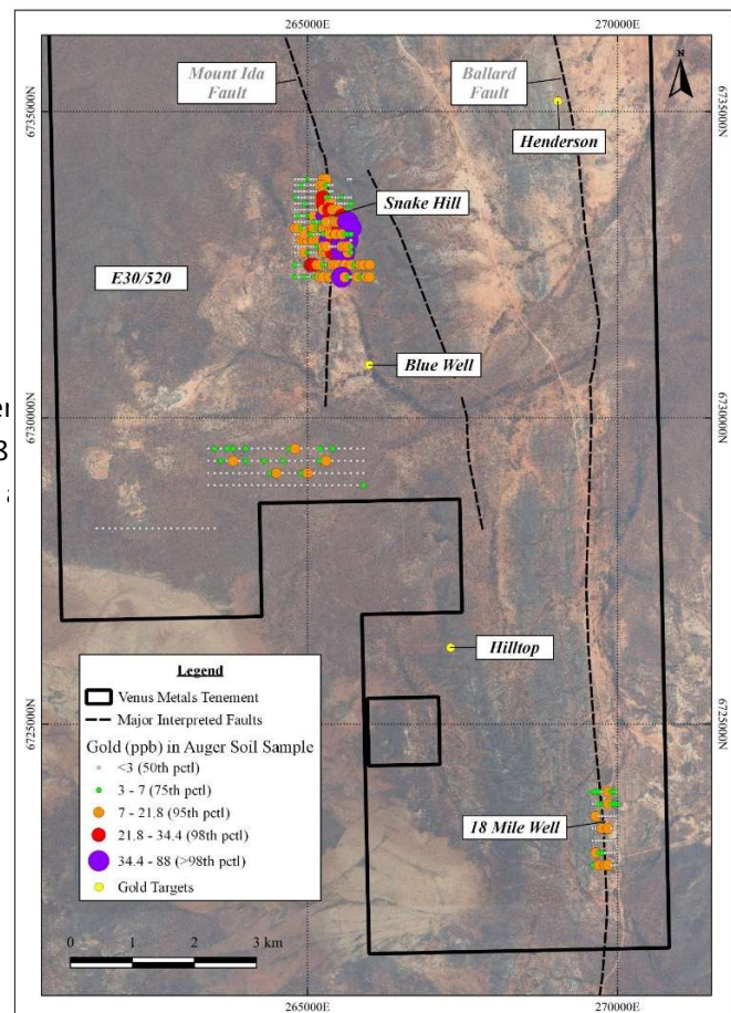
Figure 3. Gold (Au) concentrations (50 th , 75 th , 95 th and 98 th percentiles and maximum value) in auger soil samples on
