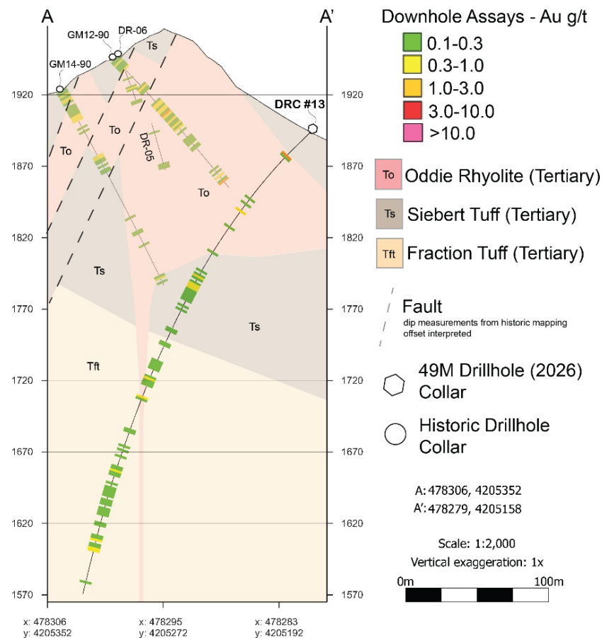
Figure 5: Cross Section of DRC#13
