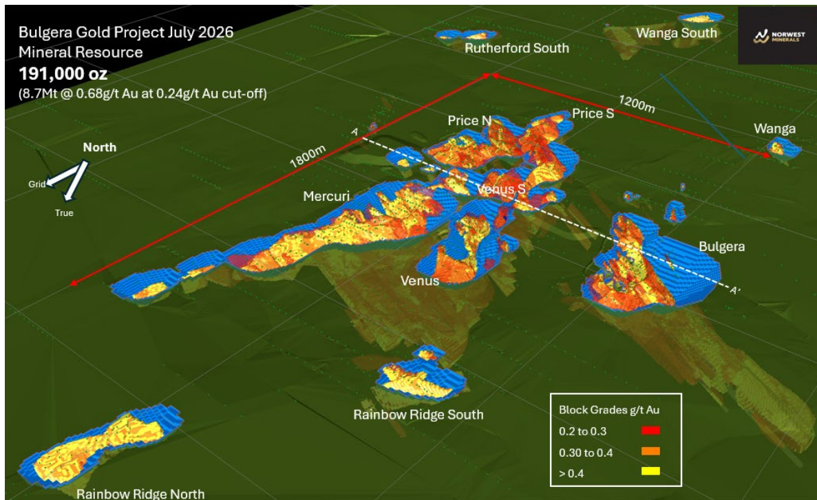
Figure 1 – Oblique view 3D representation of the July 2026 Bulgera Gold Resource model and A$5000/oz RPEEE constraining open pit(s) shell. Mineral Resource reported within the open pits only. Indicated and Inferred Mineral Resource blocks >0.20g/t Au illustrated. Oblique grid dimensions 500m x 500m.
