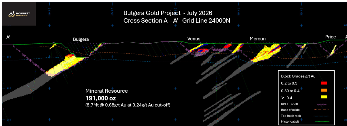
Figure 2 – Block model cross-section A-A' on Figure 1 showing gold grade as blocks >0.20g/t Au. Blocks shown represent Indicated and Inferred Mineral Resource. Unclassified Mineralisation in shaded blocks below the July 2026 Mineral Resource RPEEE shell demonstrates future Resource potential.
