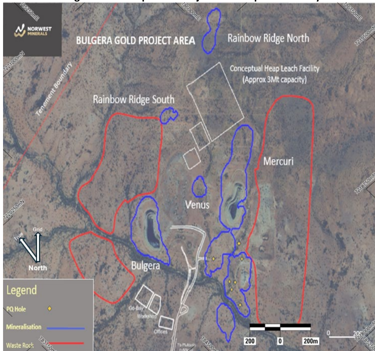
Figure 7 – Bulgera Gold heap leach conceptual design showing PQ core locations, heap leach infrastructure, areas of surface gold mineralisation, and proposed waste storage areas.
