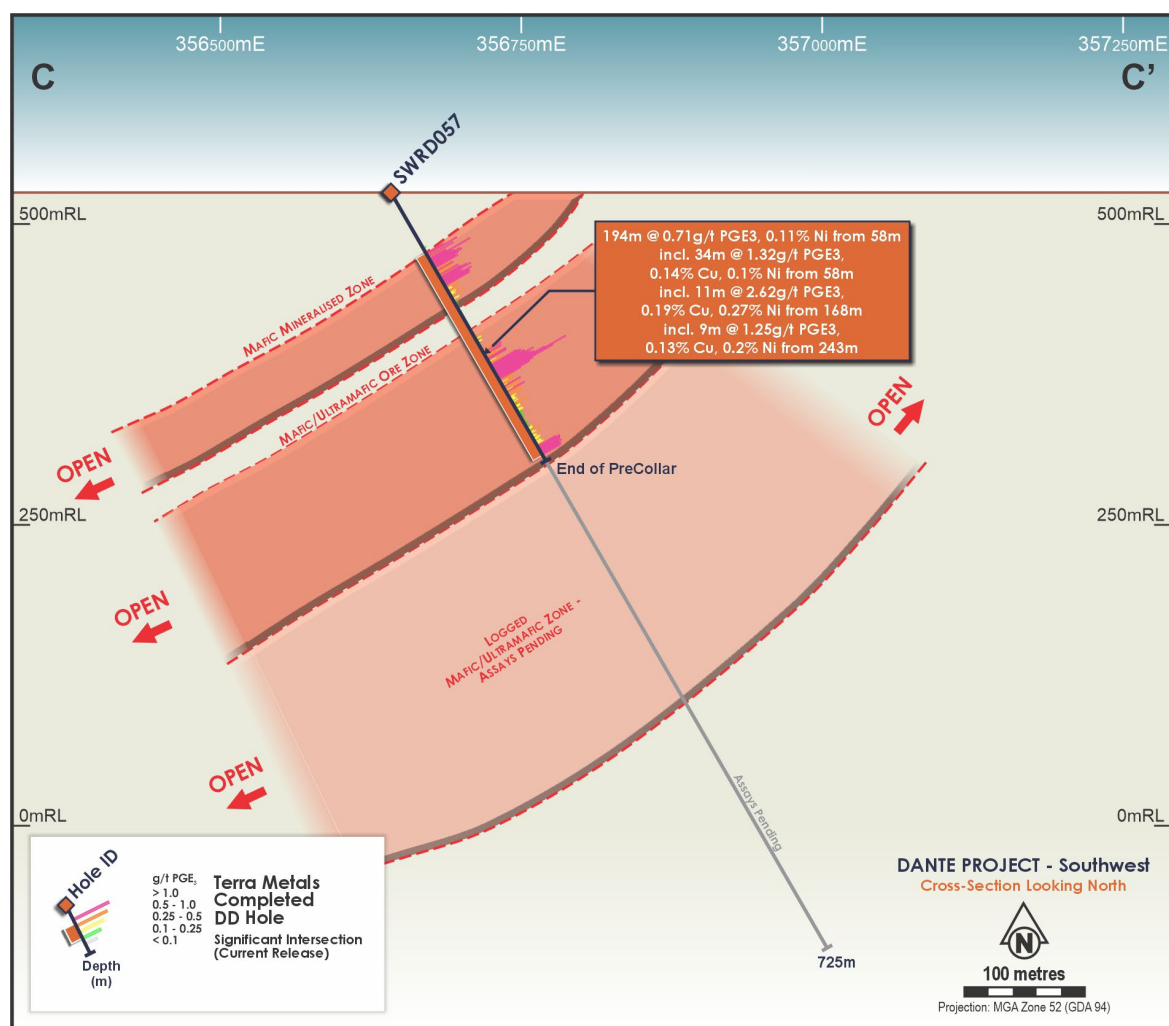
Figure 1. Cross-section C-C' through the Southwest Main Sulfide Zone including the assayed RC pre-collar and deeper diamond tail (assays pending), together with interpreted mineralised envelopes. The envelopes are conceptual and based on current drilling, geological logging and structural data.
