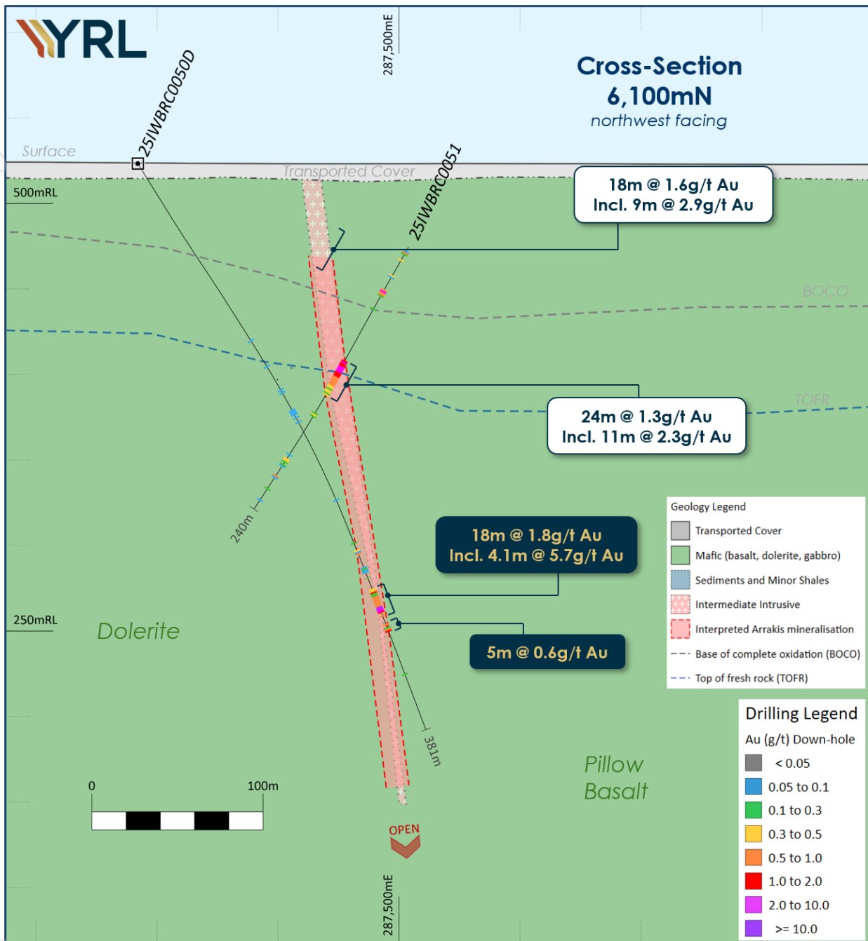
Figure 2: 6,100mN cross-section showing the completed section and all drilling results from 25IWBRC0050D. The section location is shown in Figures 4 and 5 . The section shows all drilling within +/- 25m of the section plane.
