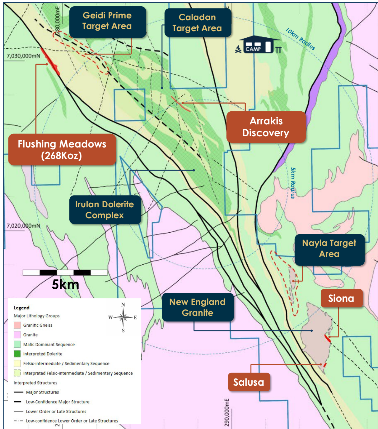
Figure 8: Yandal Resource exploration target areas and prospect locations within the northern Yandal Greenstone Belt. The Arrakis Prospect is located within the Caladan target area.
