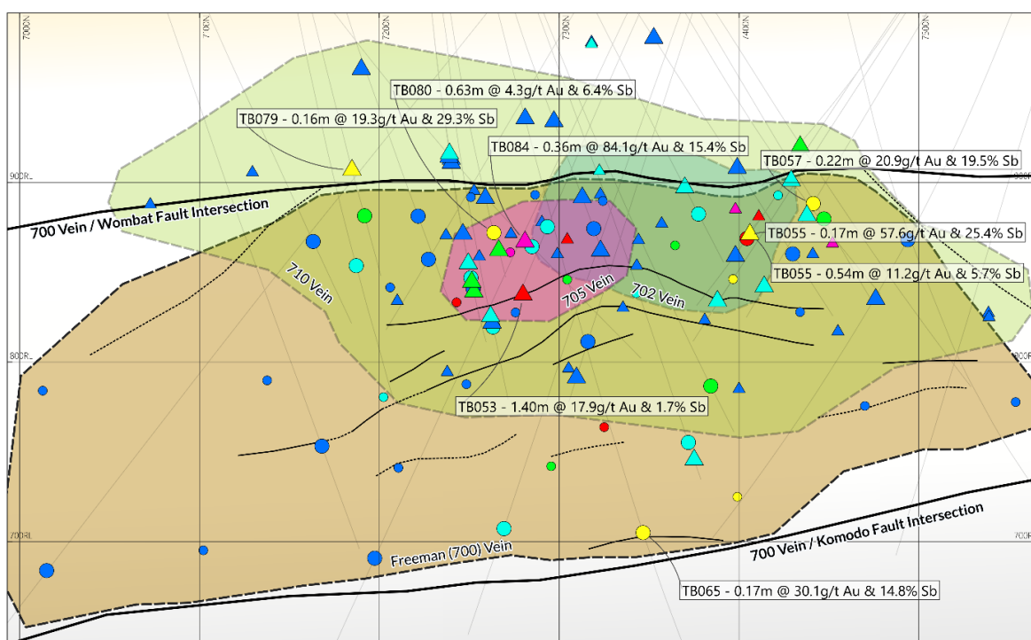
True Blue Project Longitudinal Section June 2026
