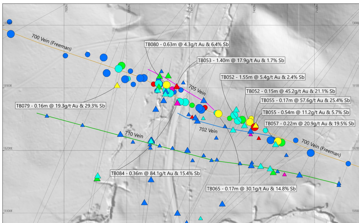
True Blue Project Plan Section June 2026
